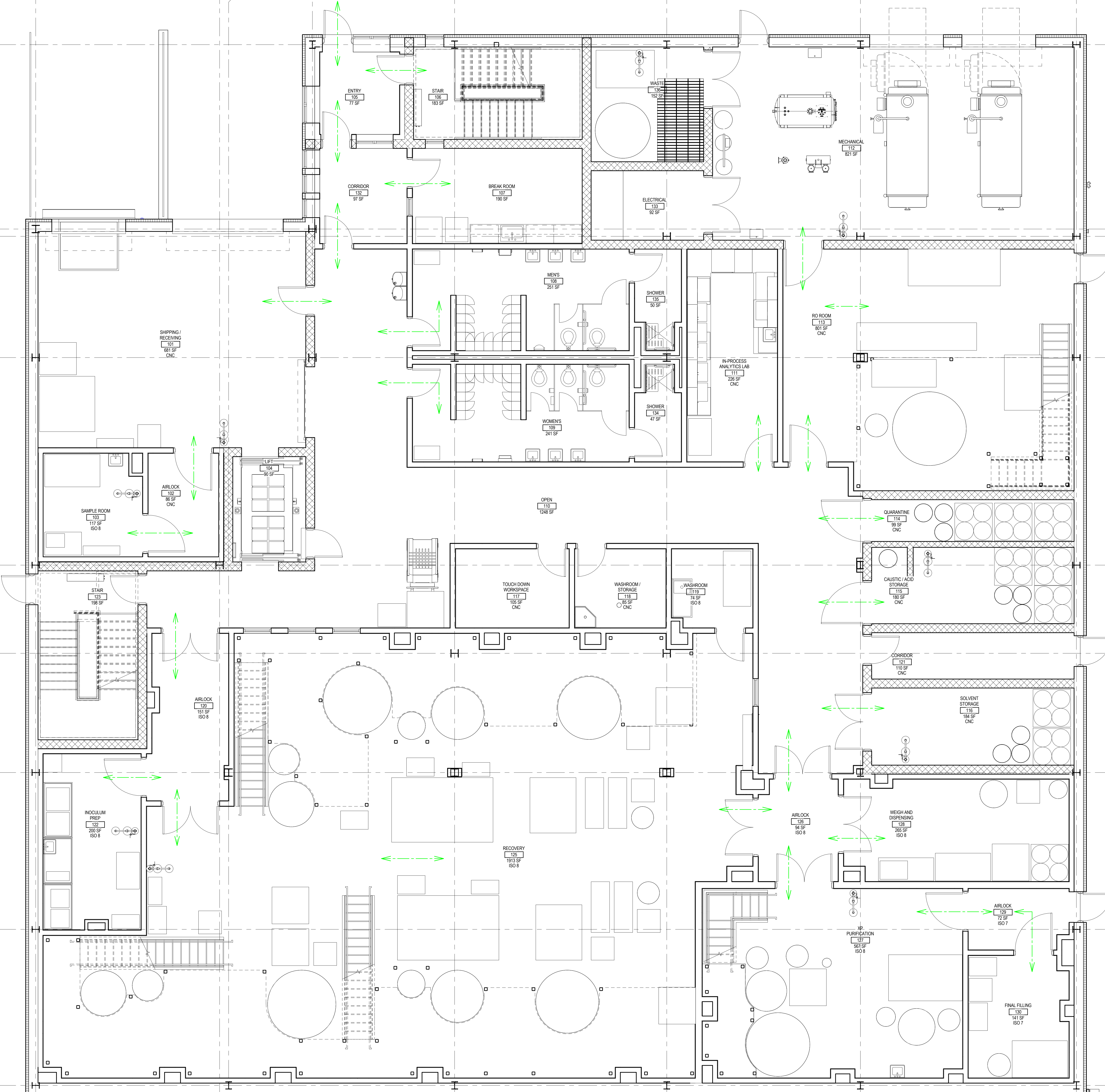
1 FIRST FLOOR PERSONNEL FLOW DIAGRAM G-106-C 1/4" = 1'-0"
