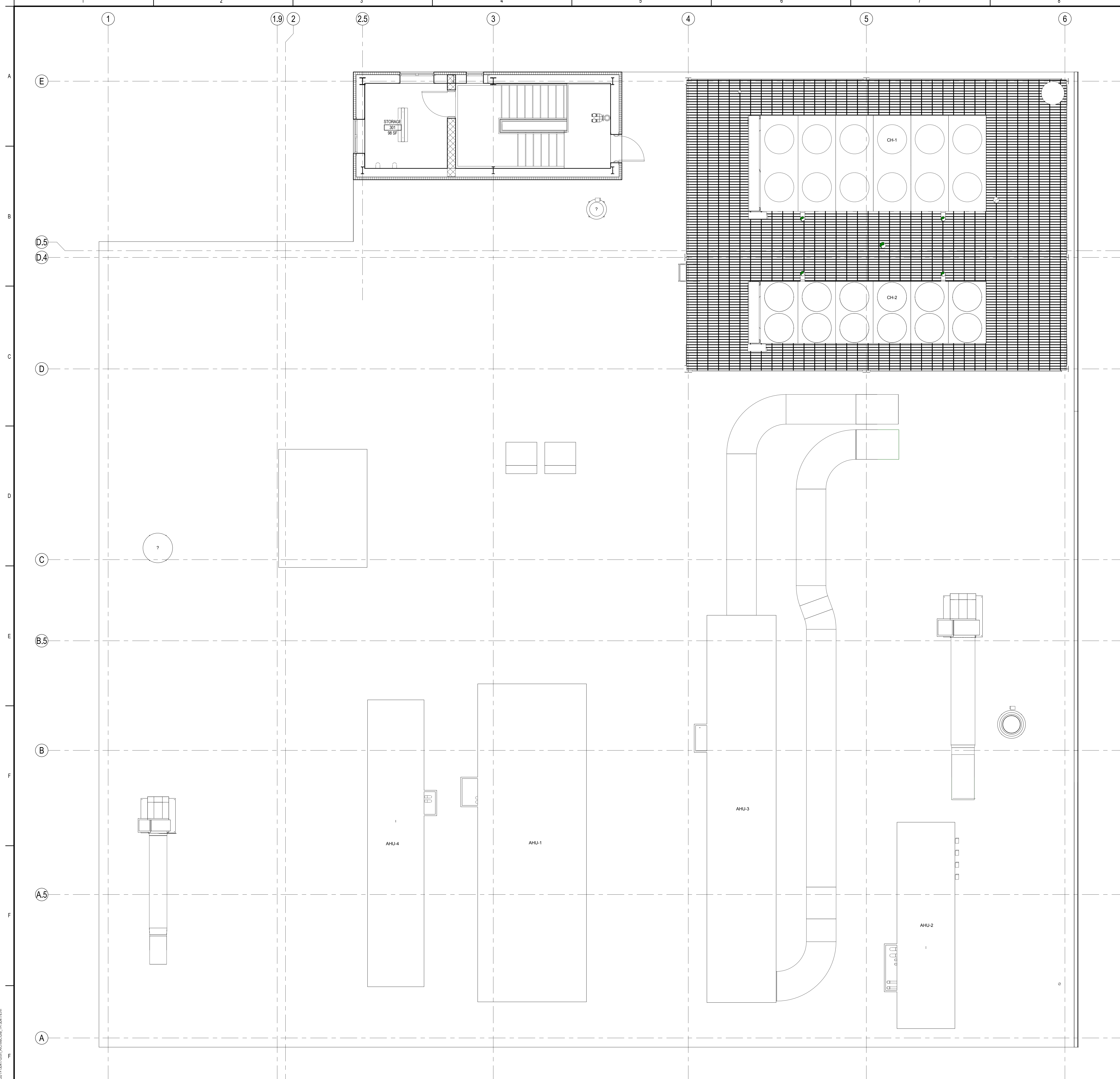
1 ROOF GENERAL ARRANGEMENT PLAN 1/4" = 1'-0"
