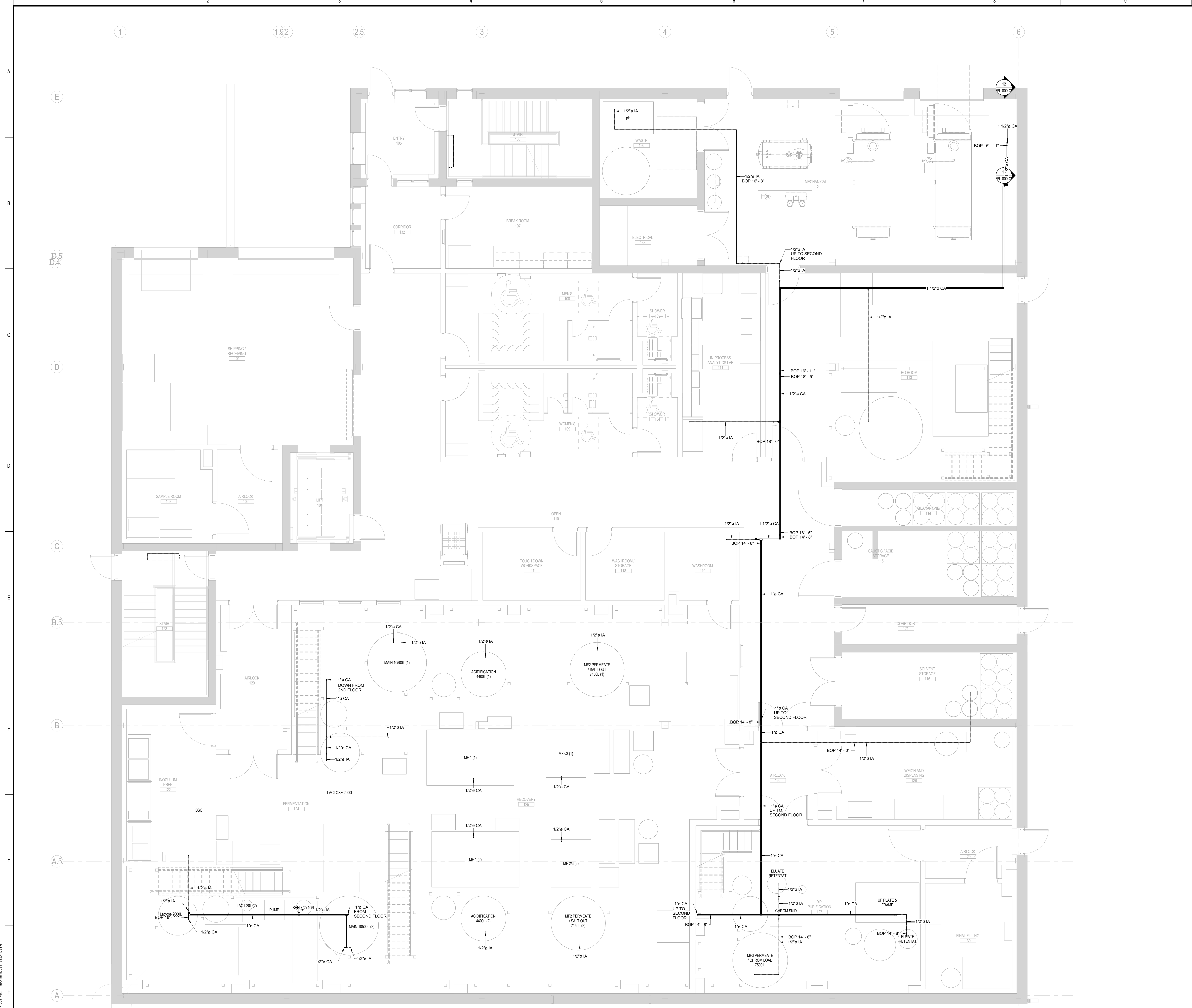
1 FIRST FLOOR - COMPRESSED AIR PIPING PLAN 1/4" = 1'-0"
