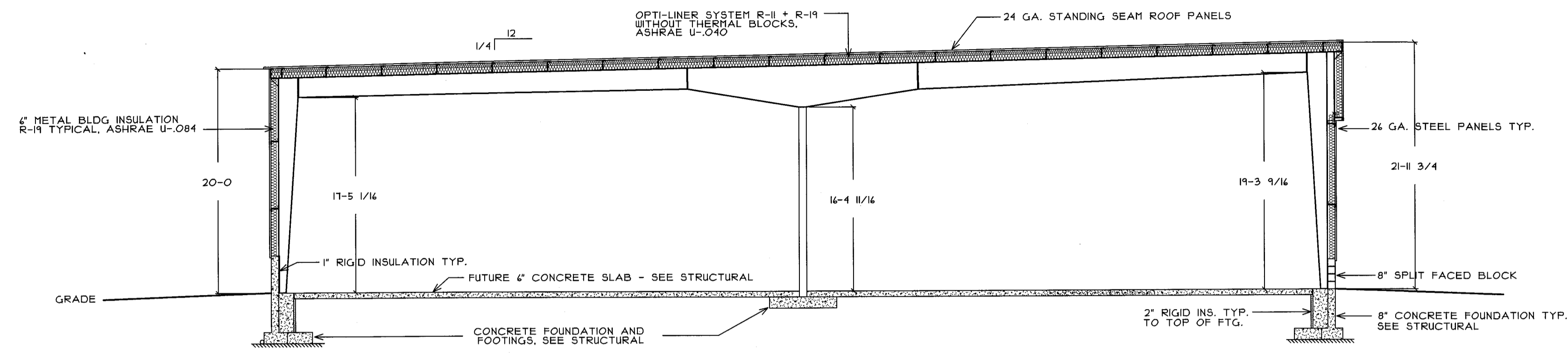
BUILDING SECTION SCALE: 1/8" = 1'-0"
