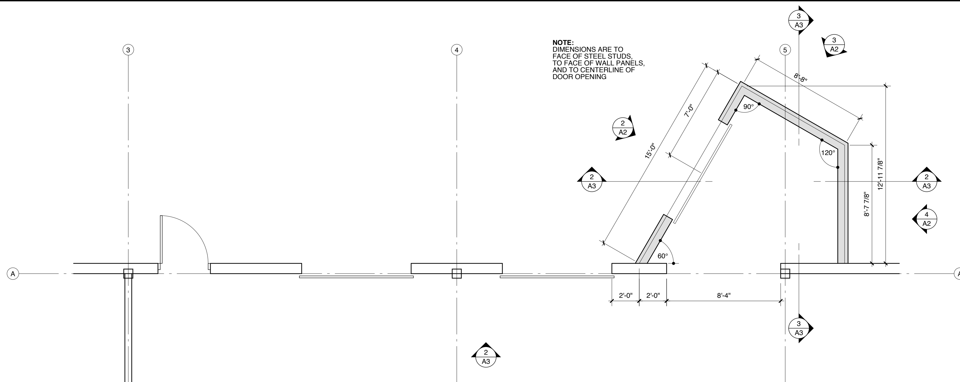
2 ENLARGED PLAN SCALE: 1/4" = 1'-0" 1' 2' 4' 8'
