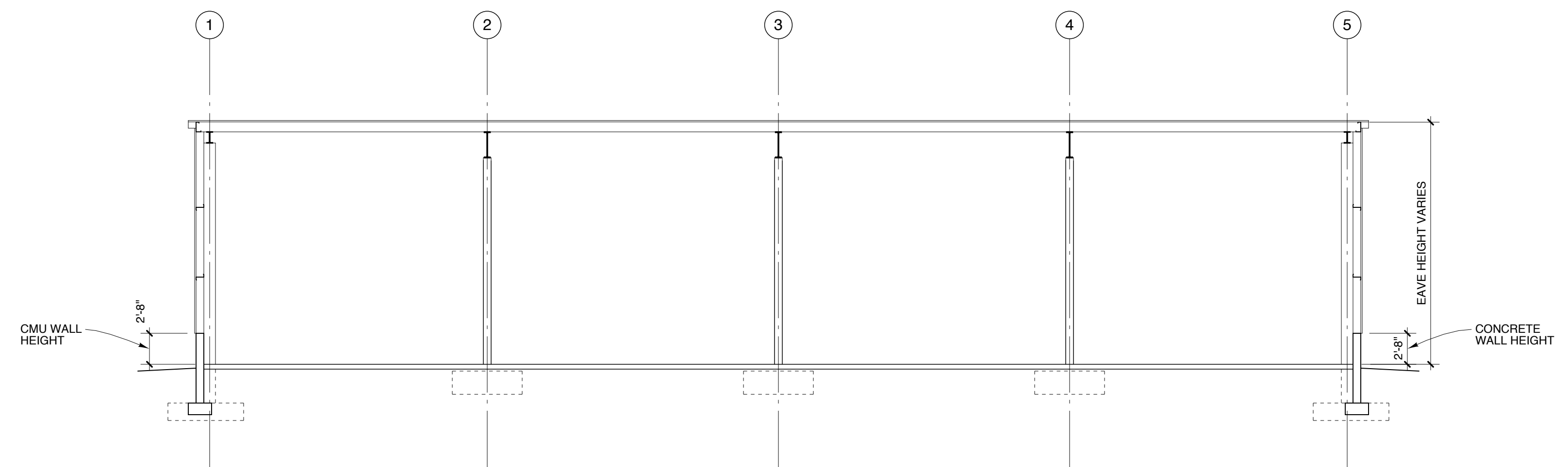
2 SECTION SCALE: 1/8" = 1'-0" 2' 4' 8' 16'
