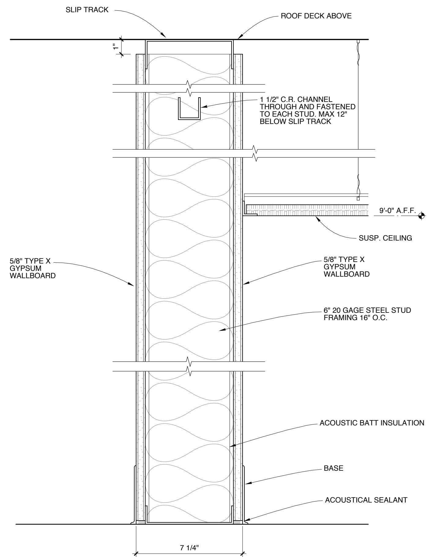
3 PARTITION TYPE P1 SCALE: 3/4" = 1'-0" 1" 2" 4" 8"
