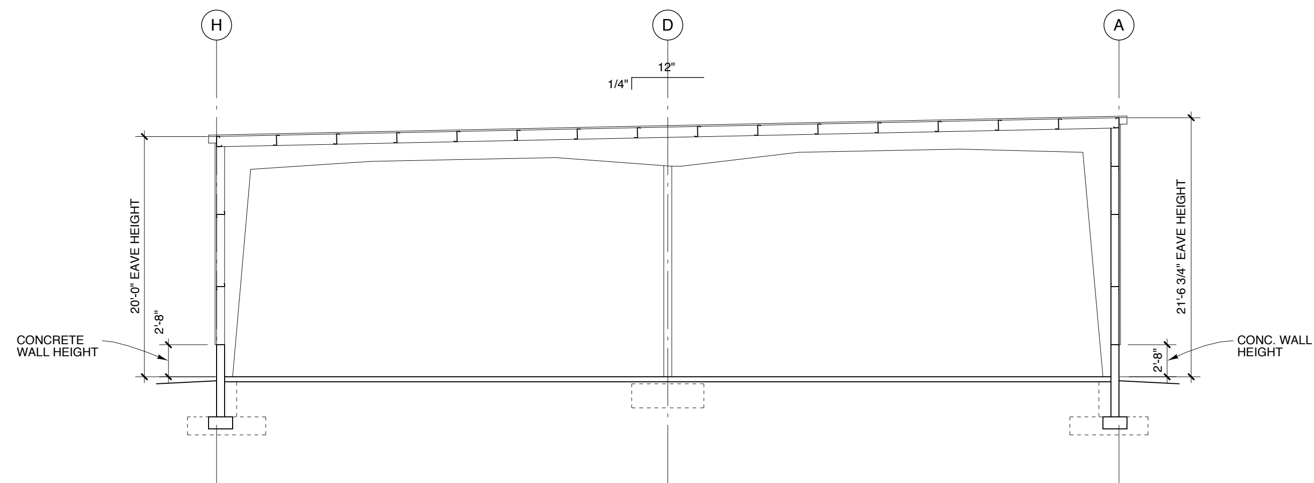
1 SECTION SCALE: 1/8" = 1'-0" 2' 4' 8' 16'
