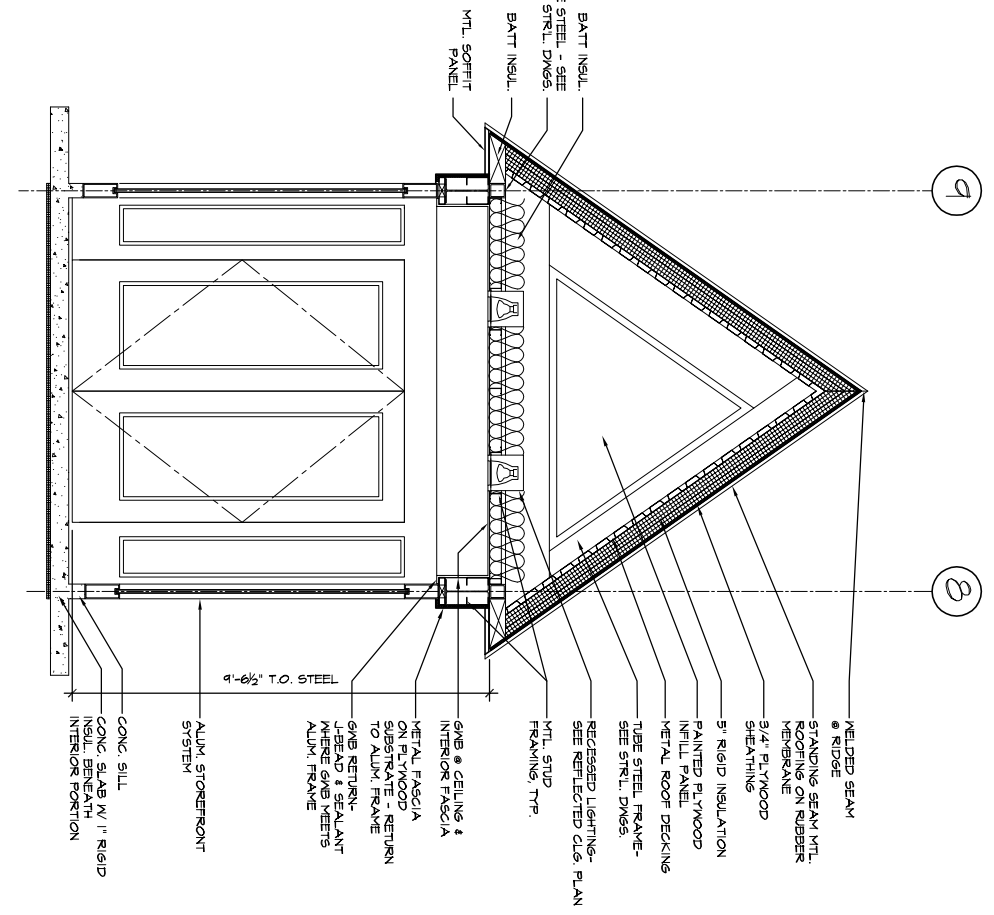
5 SECTION @ ENTRY VESTIBULE 1/2" = 1'-0"
