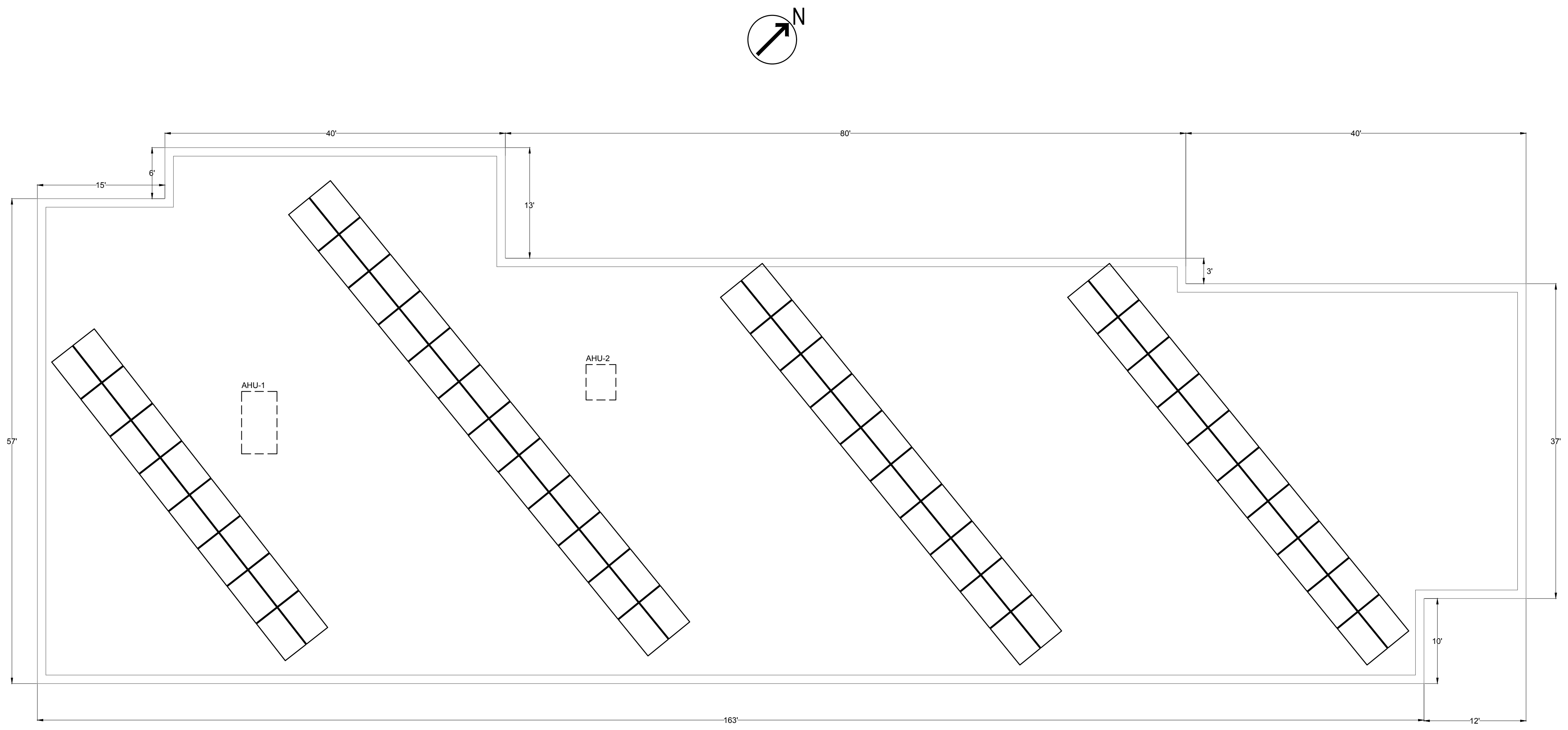
1 SOLAR PANEL LAYOUT - BUILDING PLAN SCALE: 1/8" = 1'-0"
