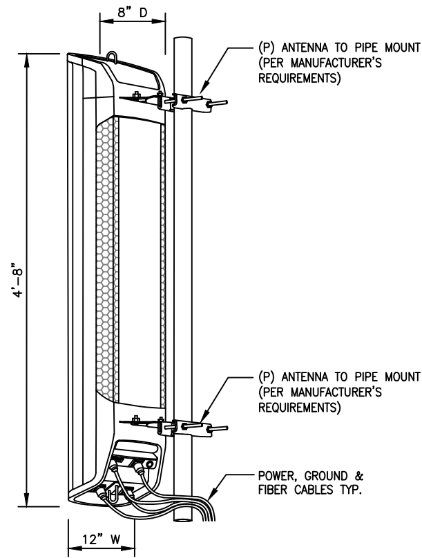
AIR21 ANTENNA TYP. 1 A-3
