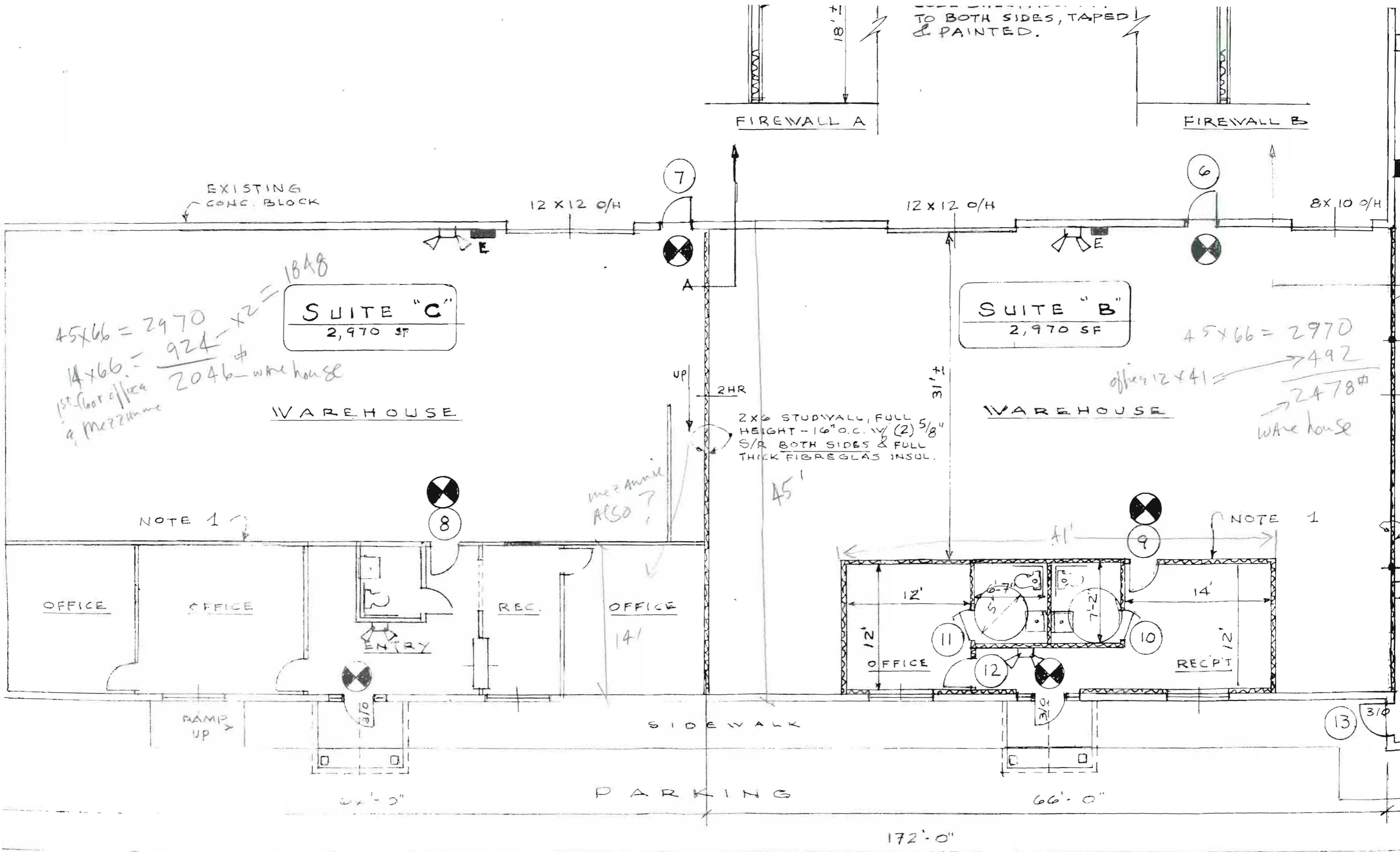
(EXISTING) ° FIRST FLOOR PLAN ° 1/8" = 1'-0" °
