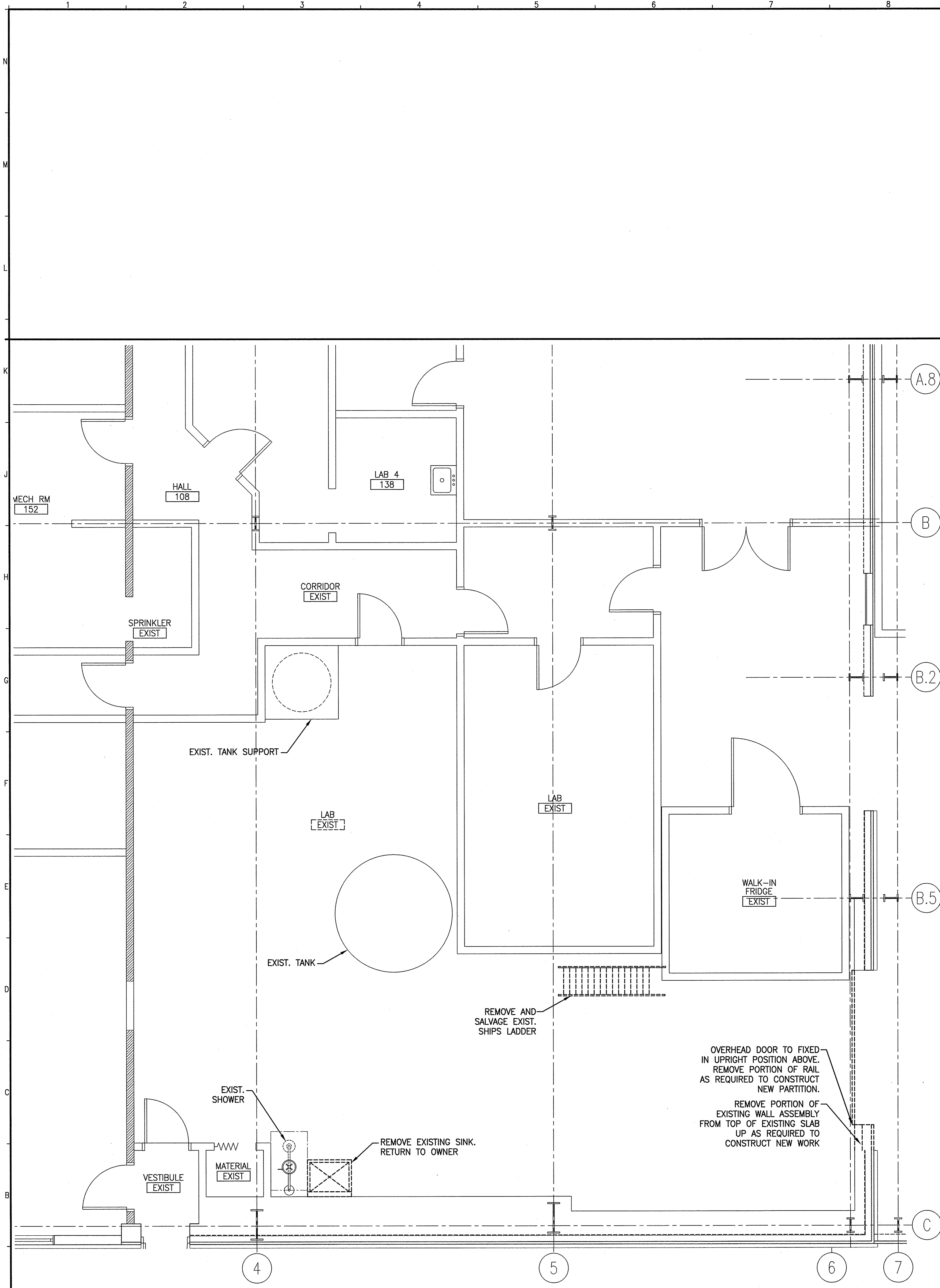
A1 FIRST FLOOR DEMOLITION PLAN
