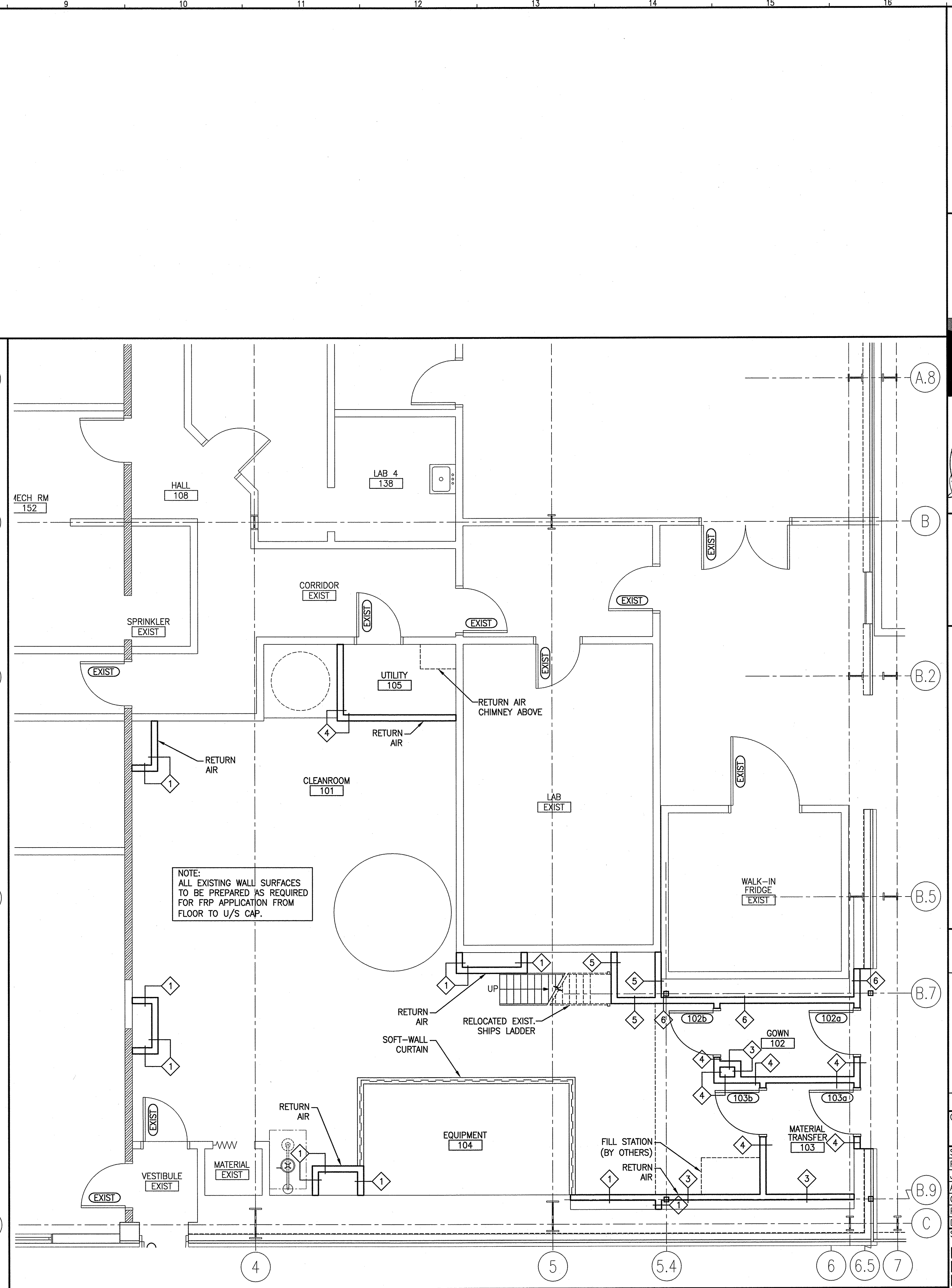
A9 FIRST FLOOR PLAN (PROPOSED)
