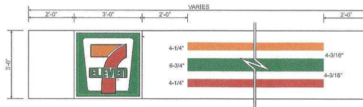
9 Front View (Typical 36" Canopy Sign & Graphic Layout) - Sign Type C 3/8" = 1'-0"
