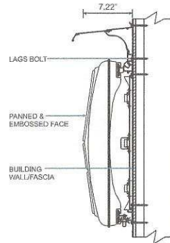
6 Side Mounting Detail - Signs B NTS
