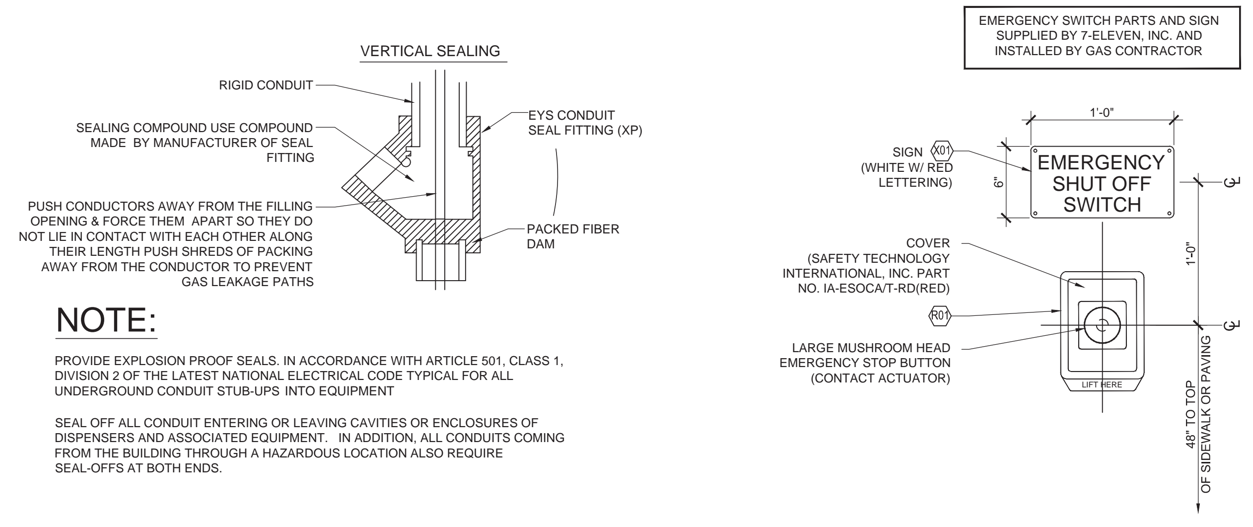
3 SEAL FITTING INSTALLATION NTS
