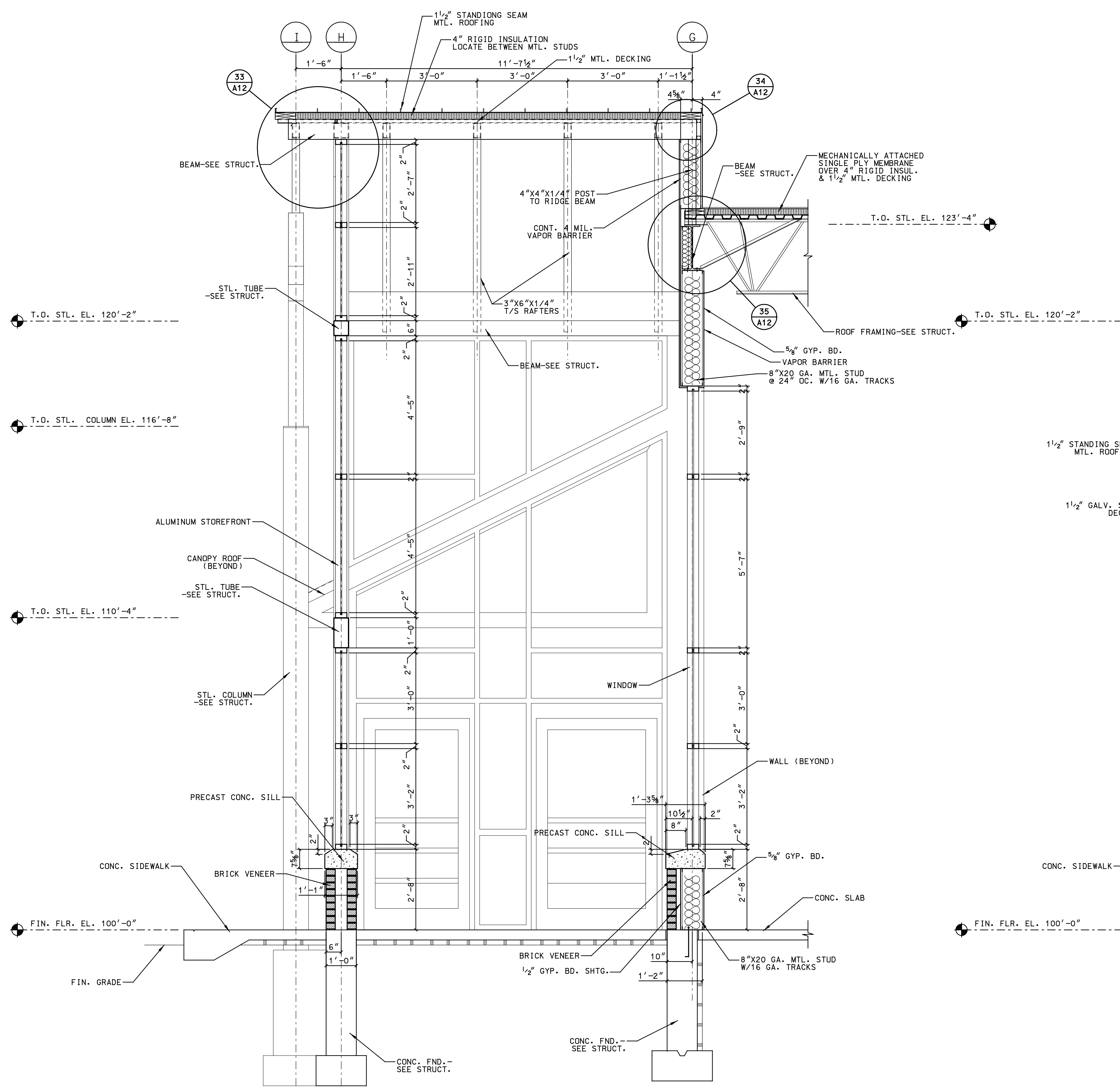
I-I WALL SECTION 1/2" = 1'-0"
