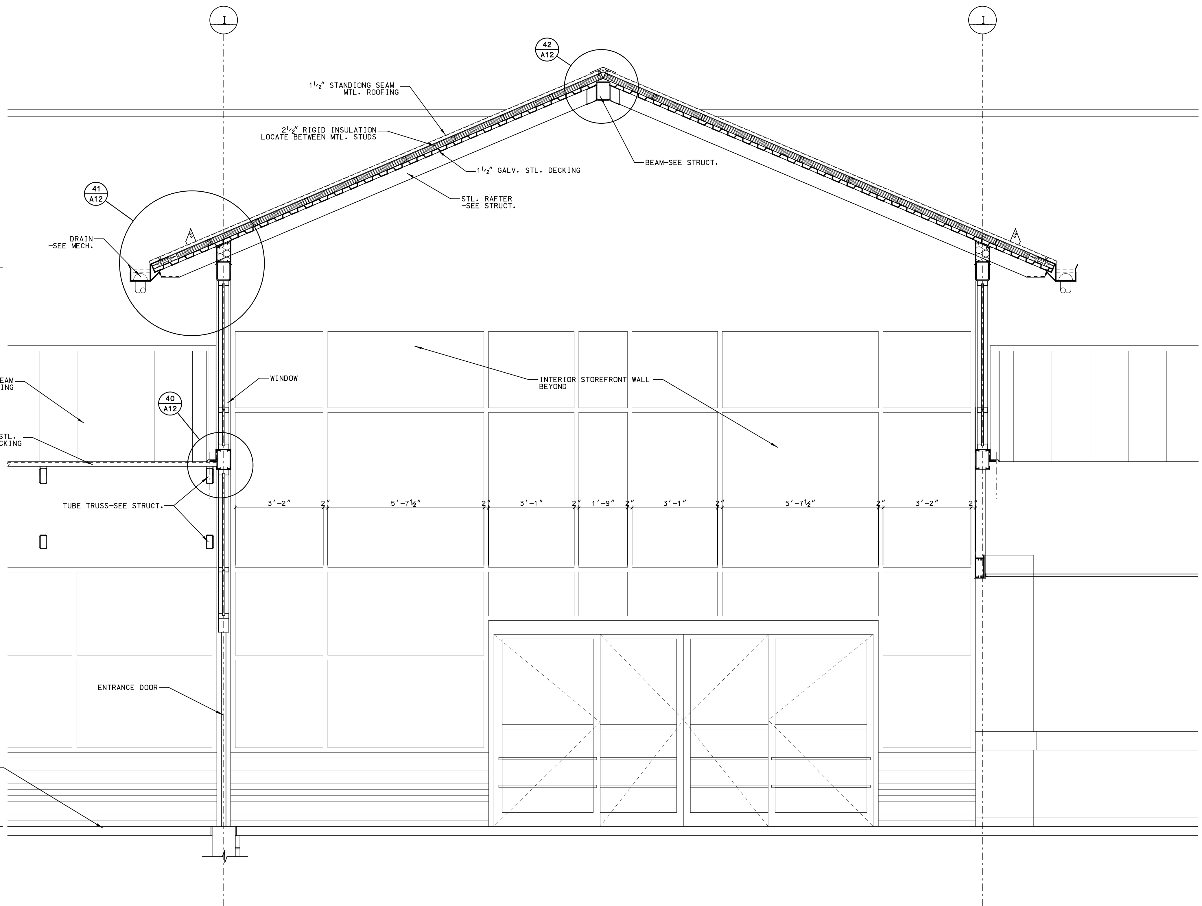
J-J WALL SECTION 1/2" = 1'-0"
