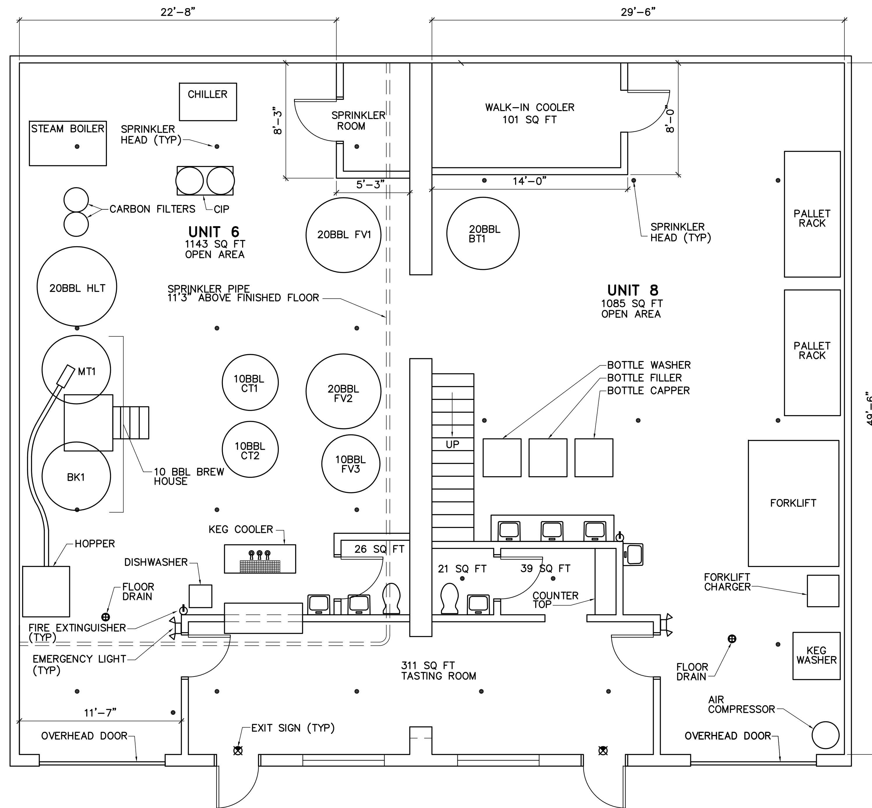
AUSTIN STREET BREWERY LAYOUT PLAN 2626 TOTAL SQ FEET
