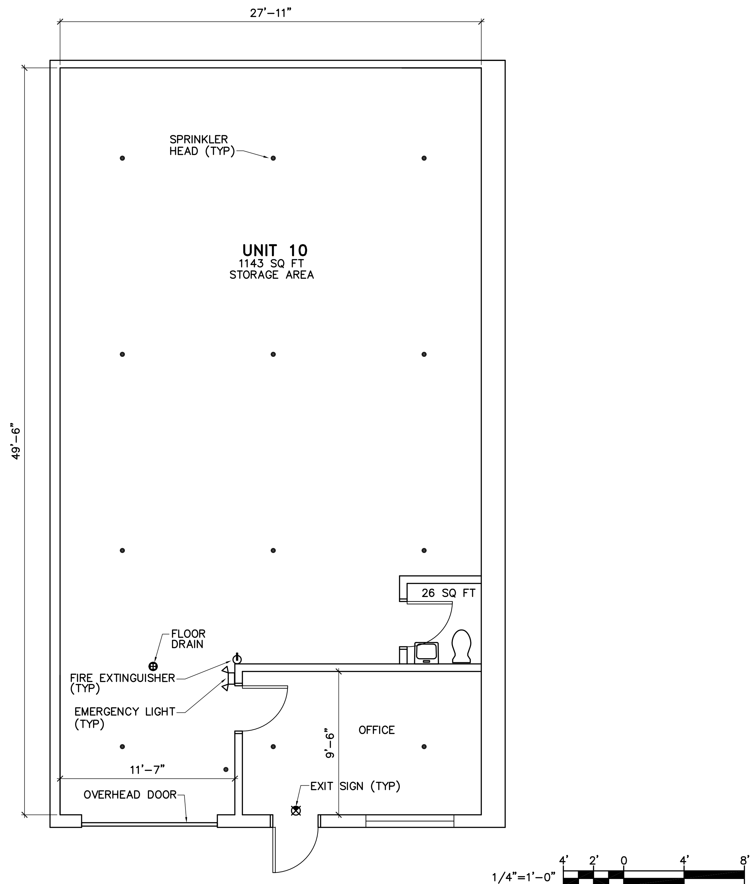
AUSTIN STREET BREWERY STORAGE LAYOUT PLAN
