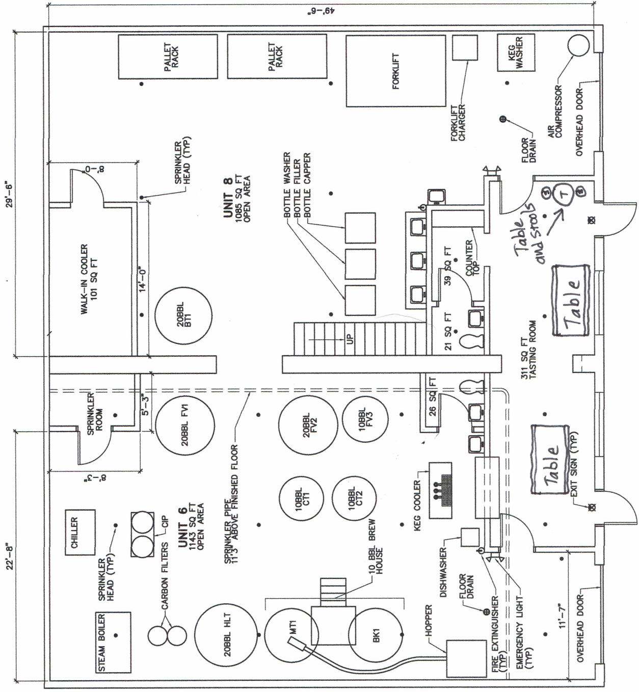
AUSTIN STREET BREWERY LAYOUT PLAN 2626 TOTAL SQ FEET
