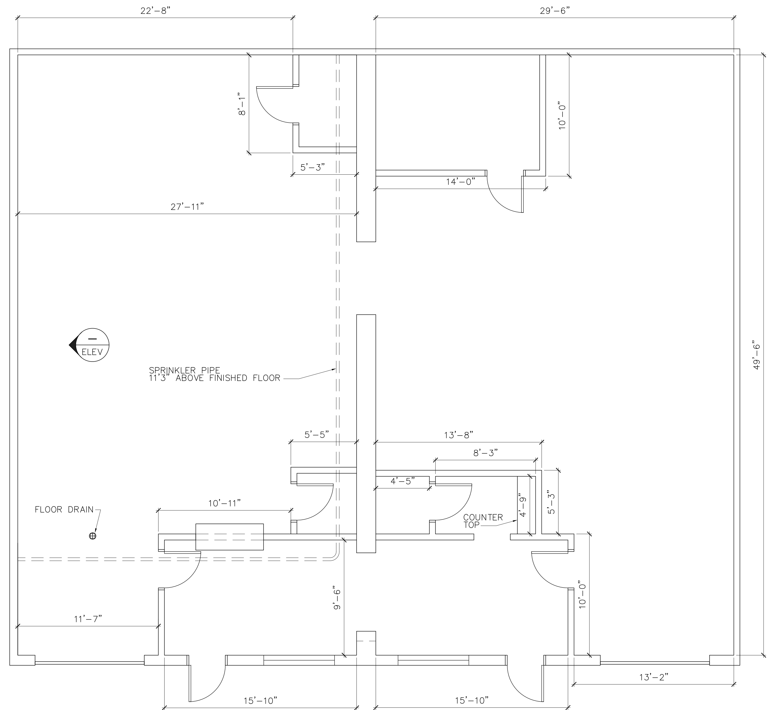
AUSTIN STREET BREWERY LAYOUT PLAN ADDITION 1380 TOTAL SQUARE FEET
