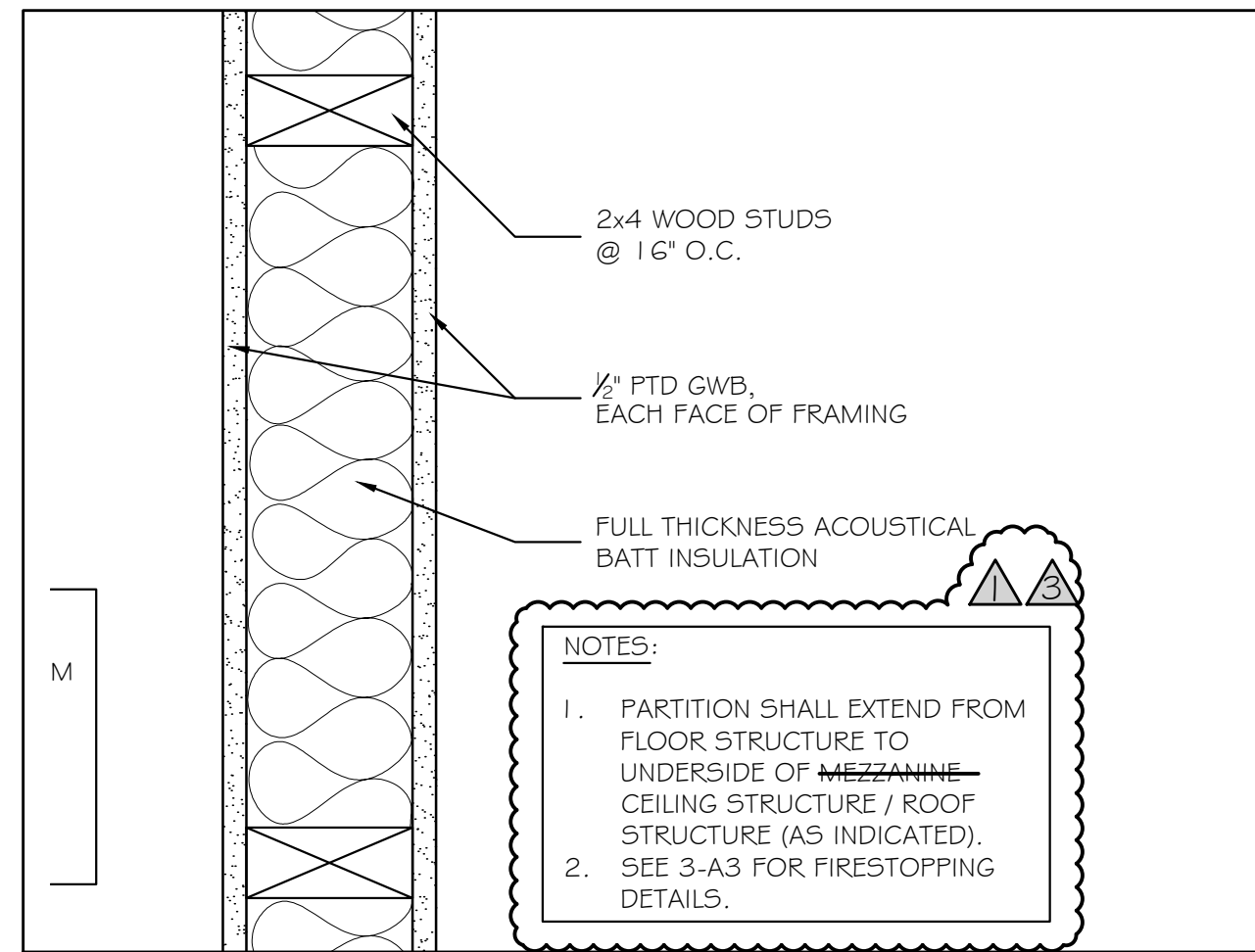
3 TYPICAL PARTITION 3" = 1'-0"
