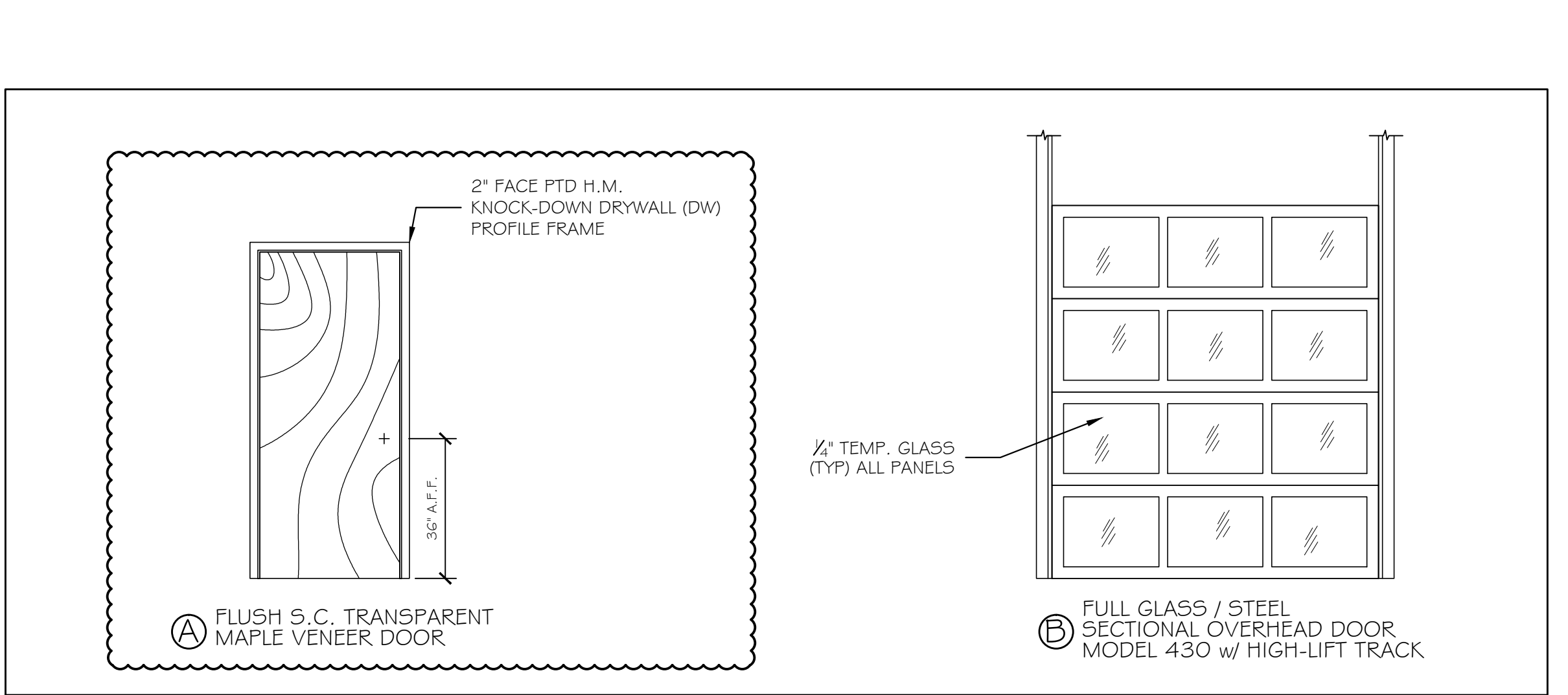
DOOR TYPES 3/8" = 1'-0"
