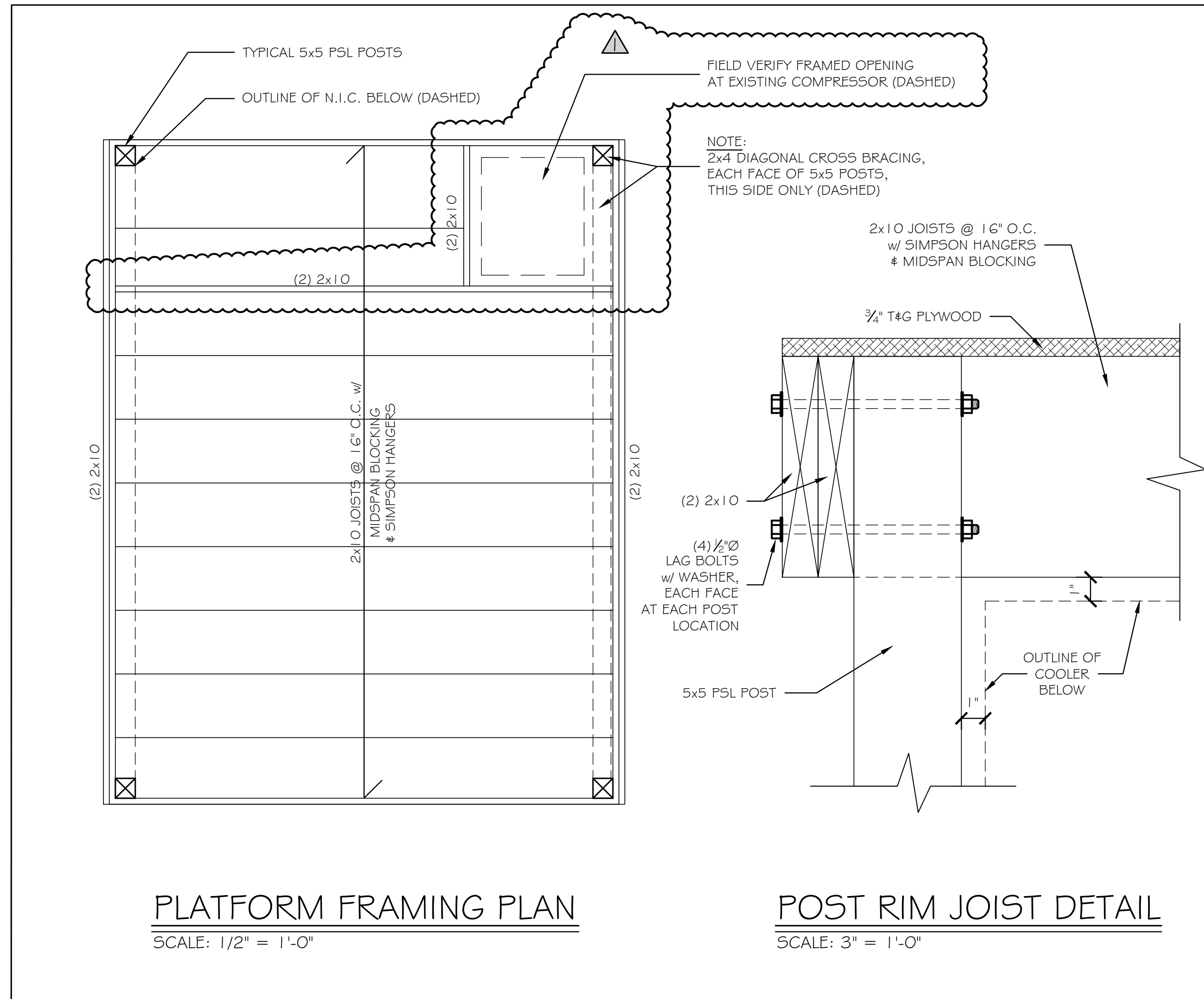
6 EQUIPMENT PLATFORM AT WALK-IN COOLER 1/2" = 1'-0"
