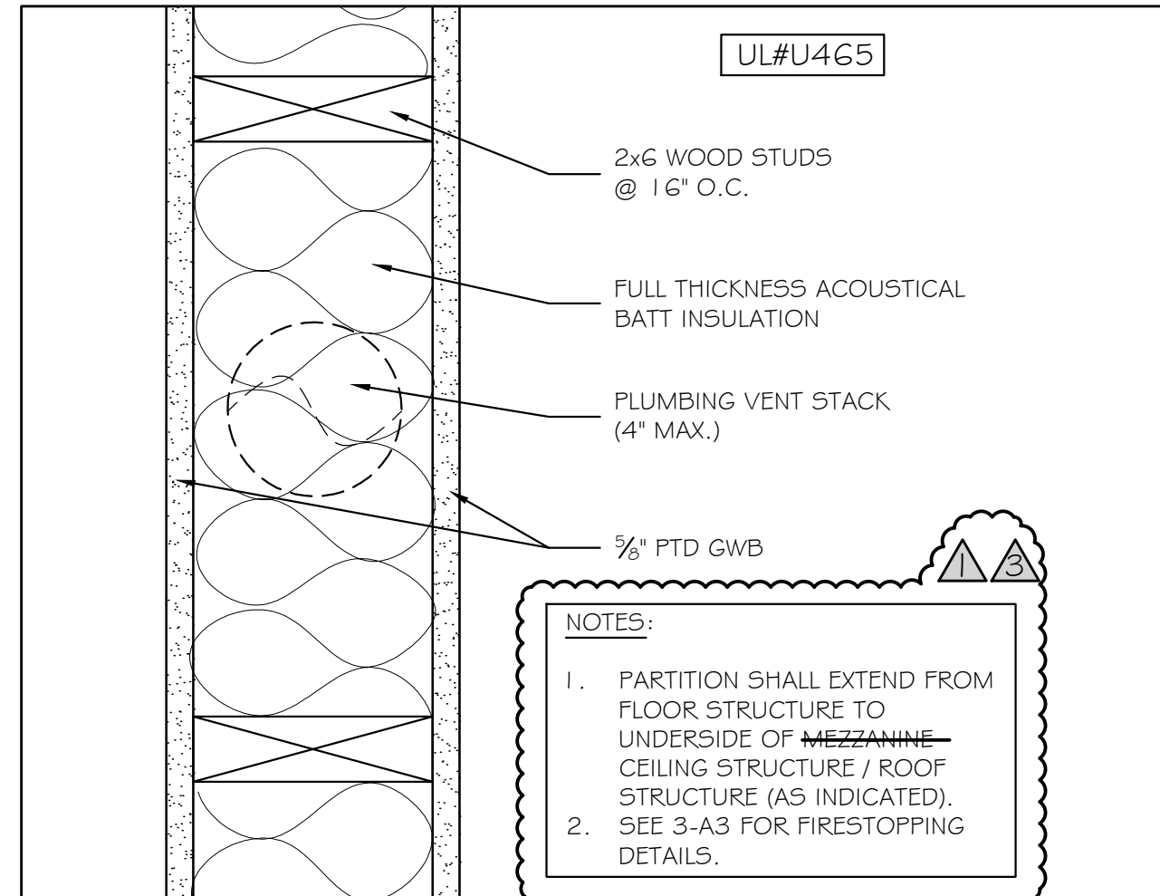
2 TYPICAL PARTITION 3" = 1'-0"
