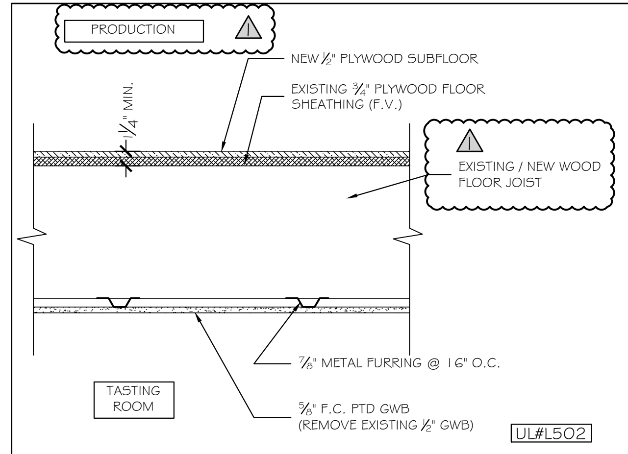
4 1 HR RATED FLOOR/CEILING ASSEMBLY 1 1/2" = 1'-0"
