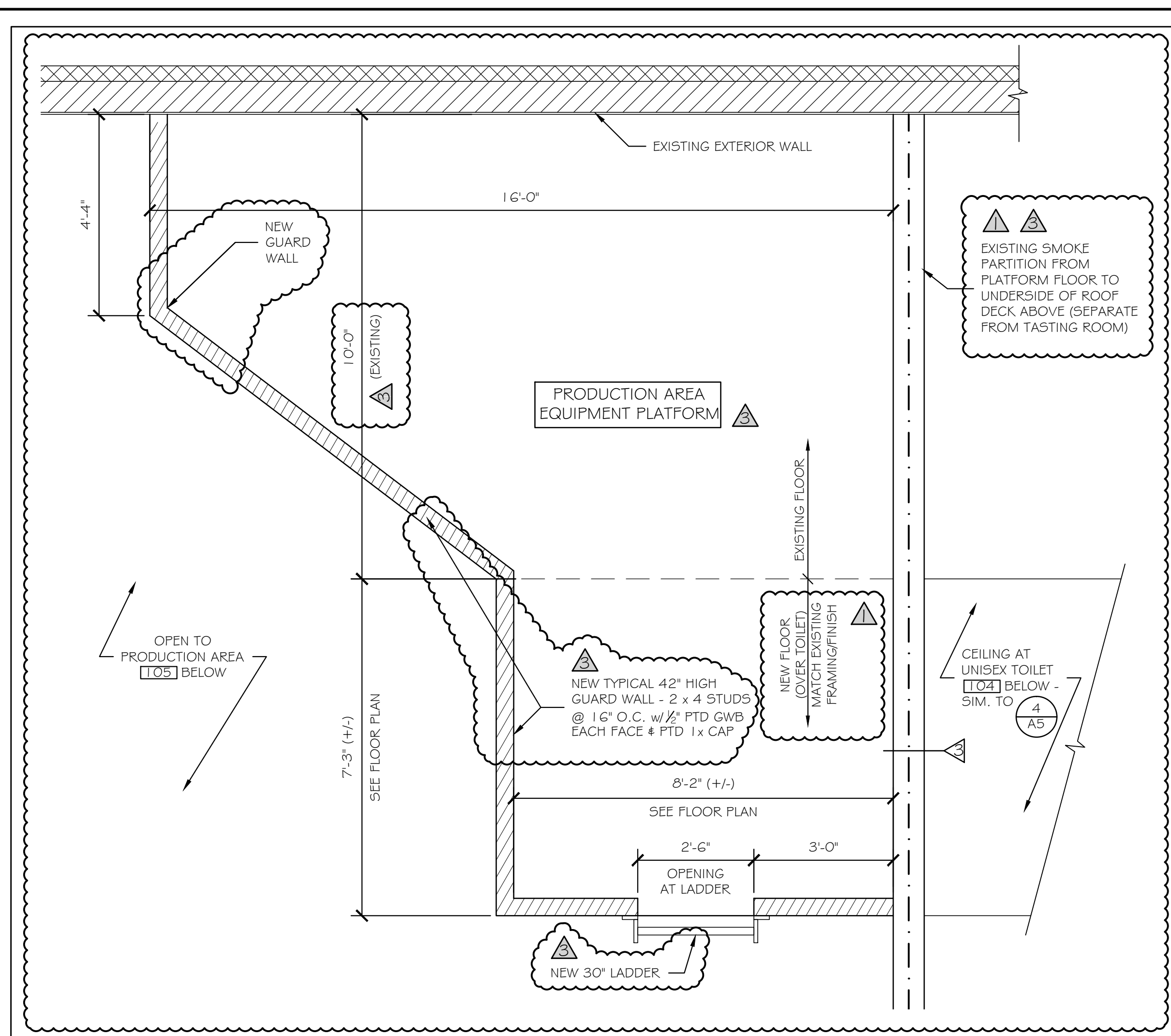
5 STORAGE MEZZANINE AT PRODUCTION AREA PLAN 1/2" = 1'-0"
