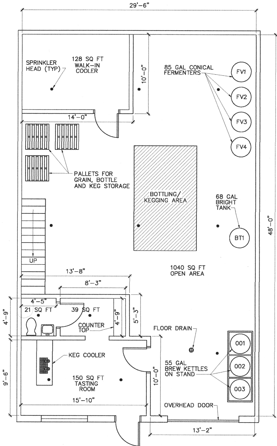
AUSTIN STREET BREWERY LAYOUT PLAN 1380 TOTAL SQUARE FEET
