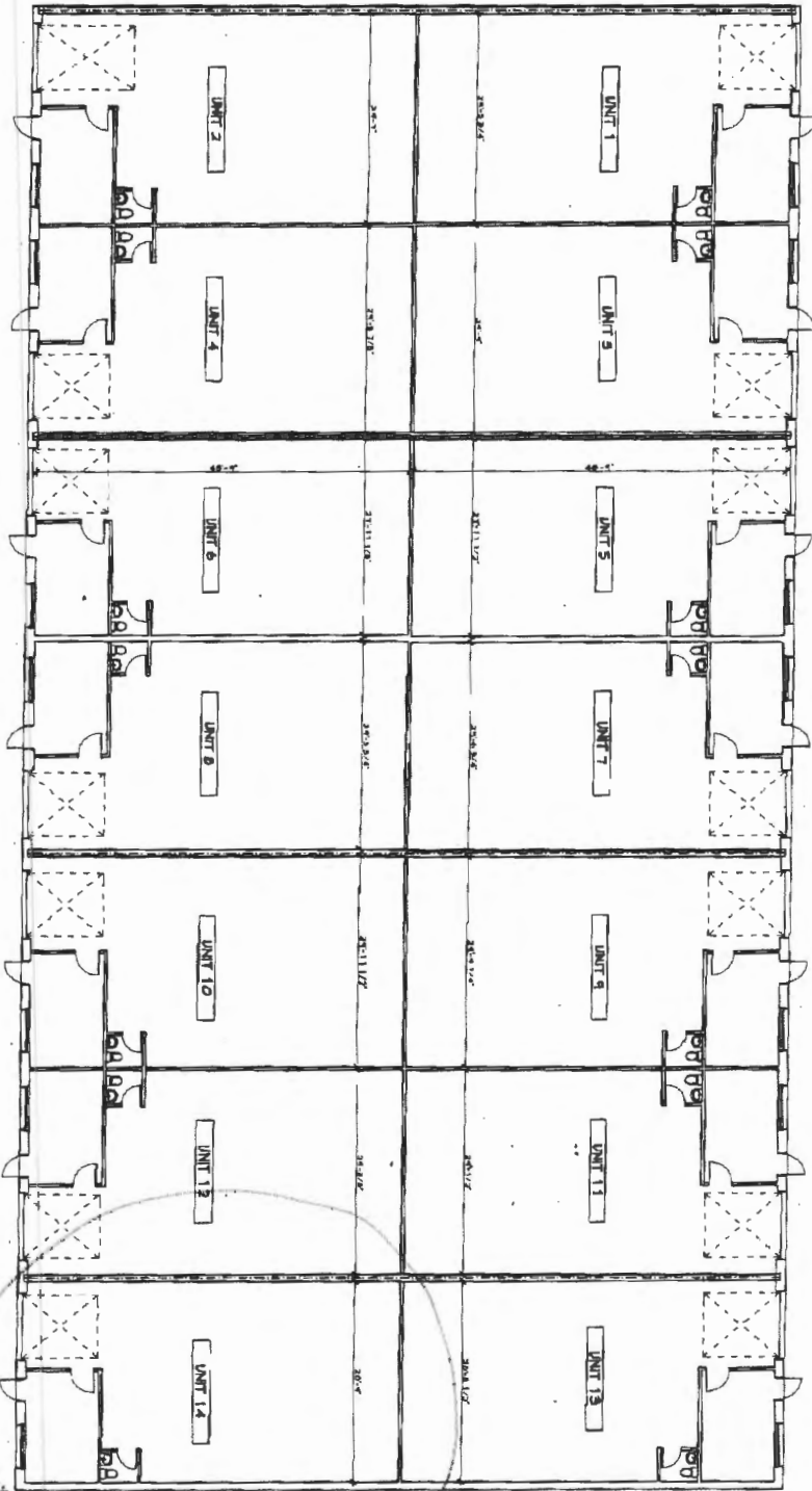
1 BUILDING FLOOR PLAN
