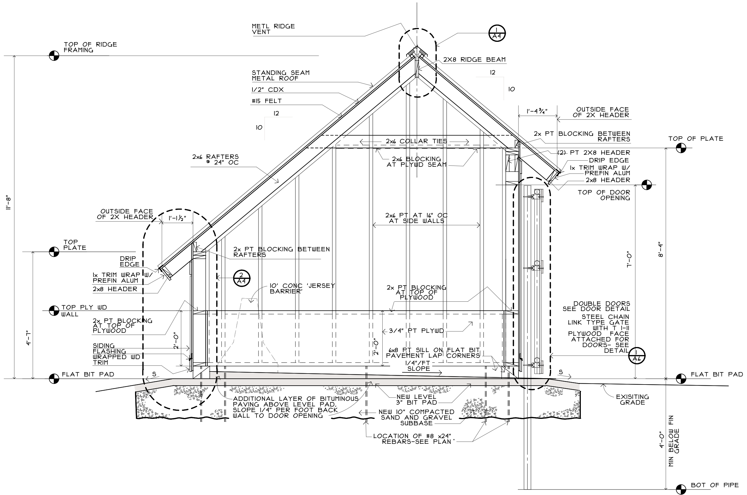
1 SECTION THRU BUILDING A3 SCALE: 1/2"=1'-0"
