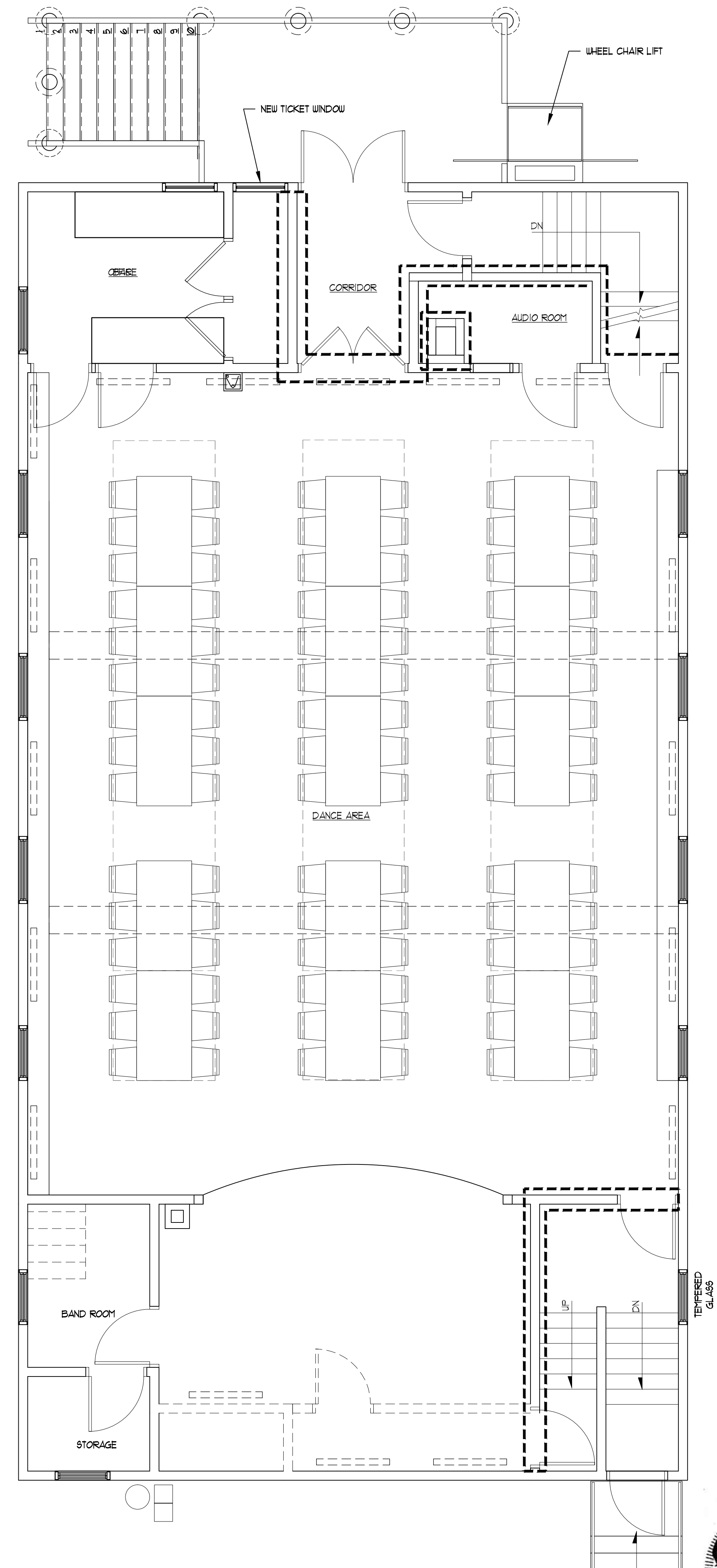
2 CONCENTRATED FSEATING (2) FIRST FLOOR (90) LS1 SCALE: 1/4" = 1'-0"
