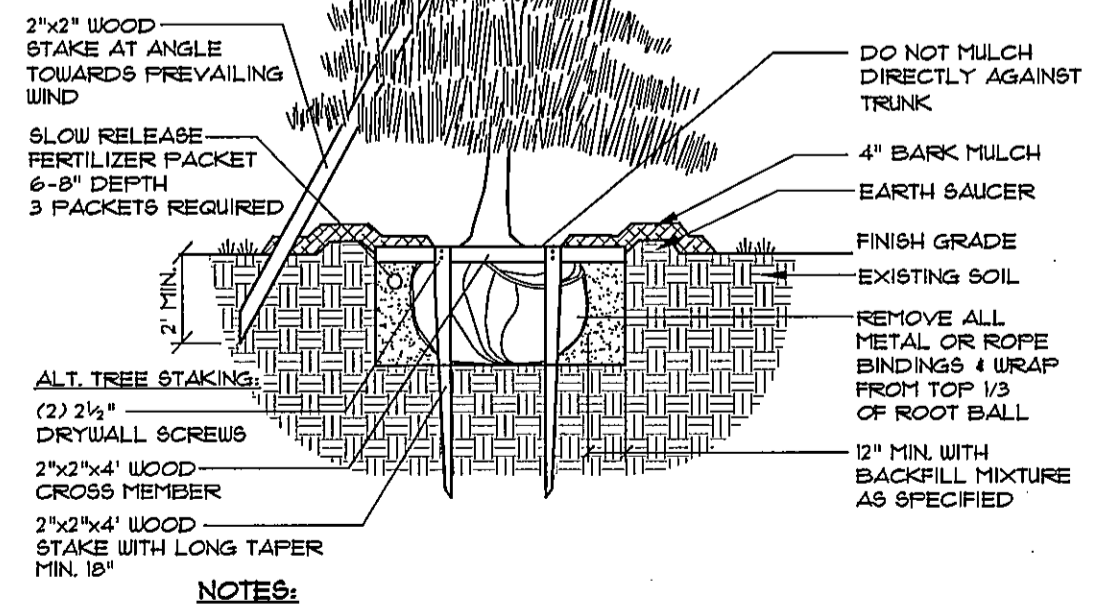
ALT. TREE STAKING PLAN NOT TO SCALE
