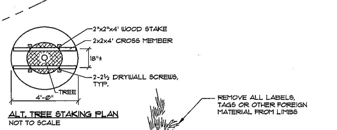
ALT. TREE STAKING PLAN NOT TO SCALE
