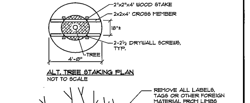
ALT. TREE STAKING PLAN NOT TO SCALE
