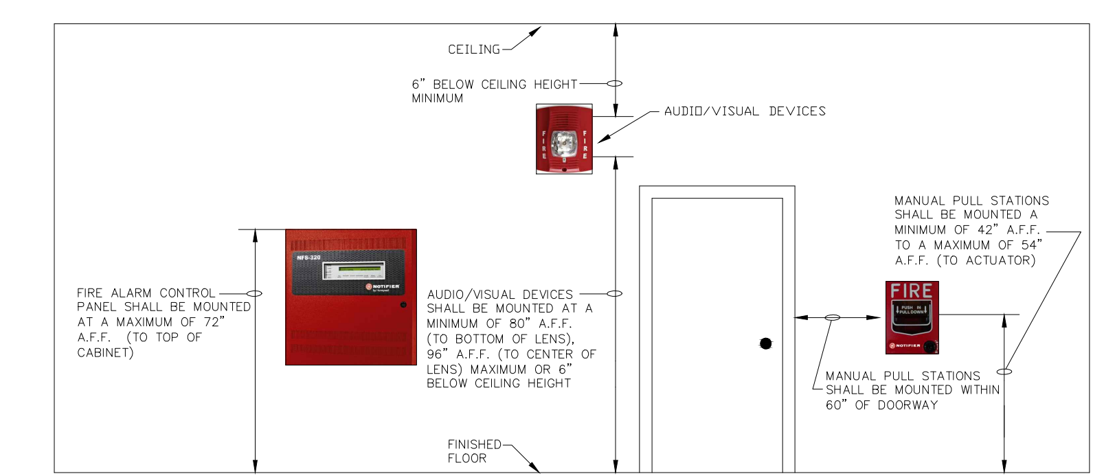
TYPICAL FIRE ALARM SYSTEM DEVICE MOUNTING HEIGHTS
