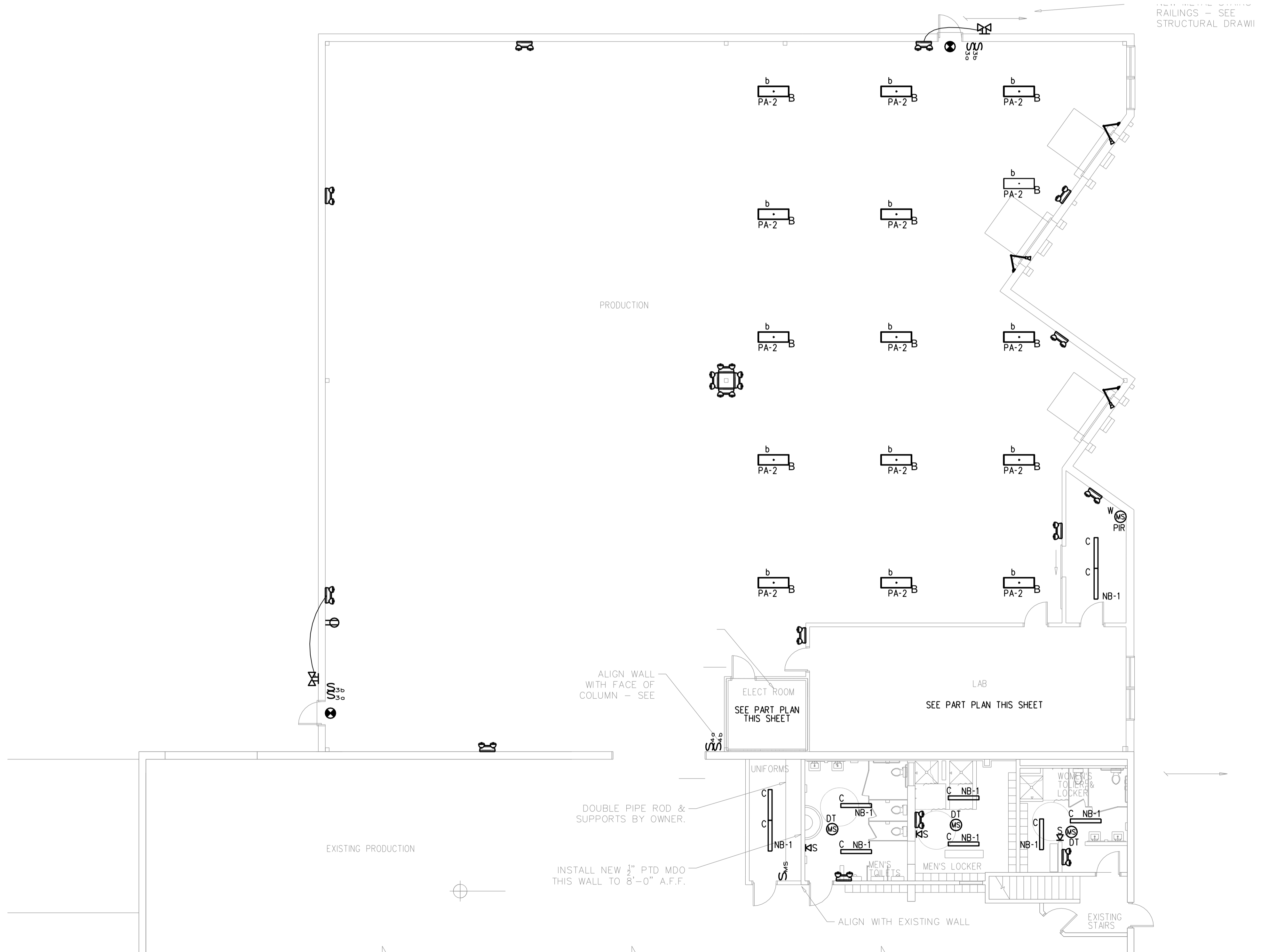
FIRST FLOOR LIGHTING PLAN SCALE: 1/8"=1'-0"
