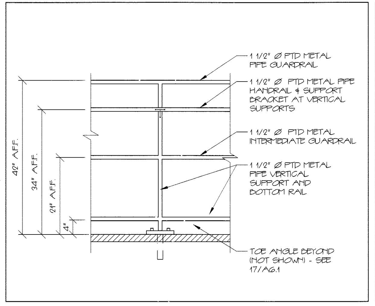
5 TYPICAL GUARDRAIL/HANDRAIL 3/4"=1'-0"
