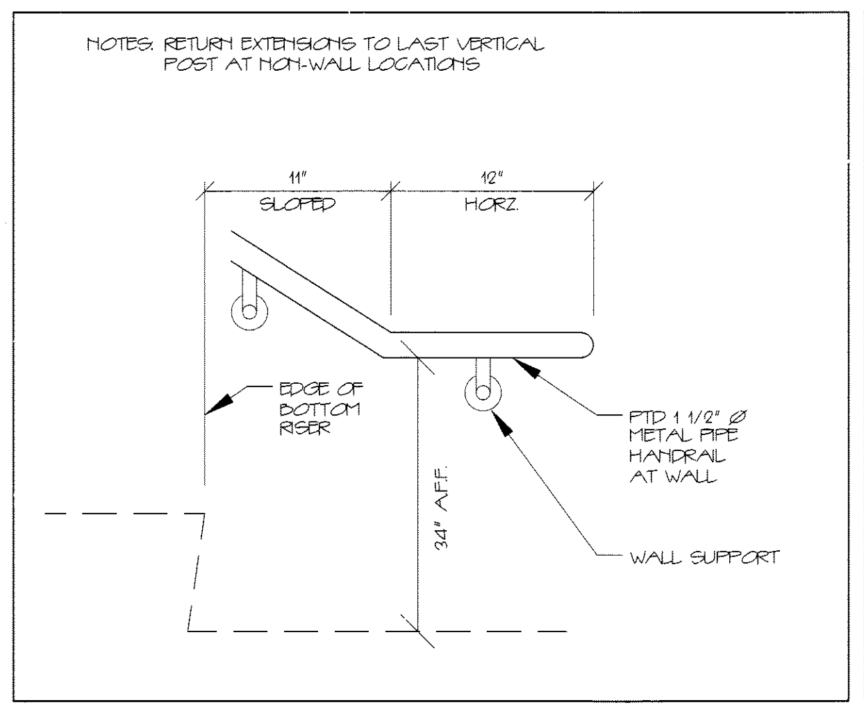
8 TYPICAL WALL HANDRAIL - BOTTOM 1 1/2"=1'-0"
