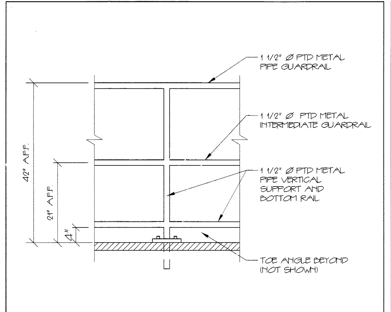
2 TYPICAL GUARDRAIL 3/4"=1'-0"
