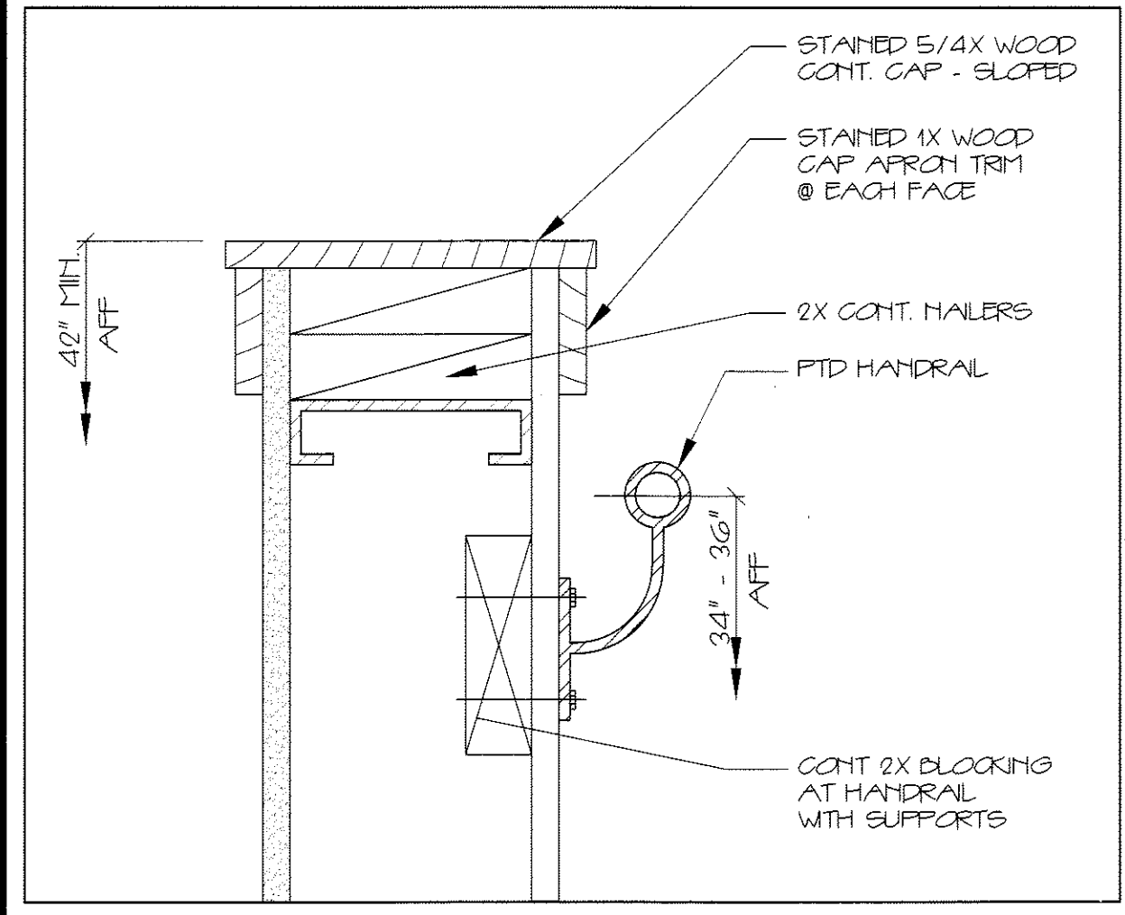
4 STAIR GUARDRAIL 3/4"=1'-0"
