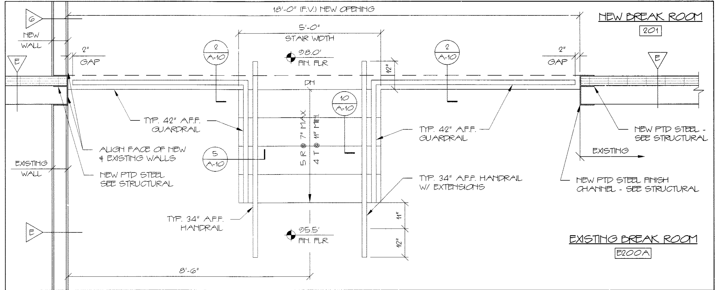
A STAR PLAN AT BREAK ROOMS 1/2"=1'-0"
