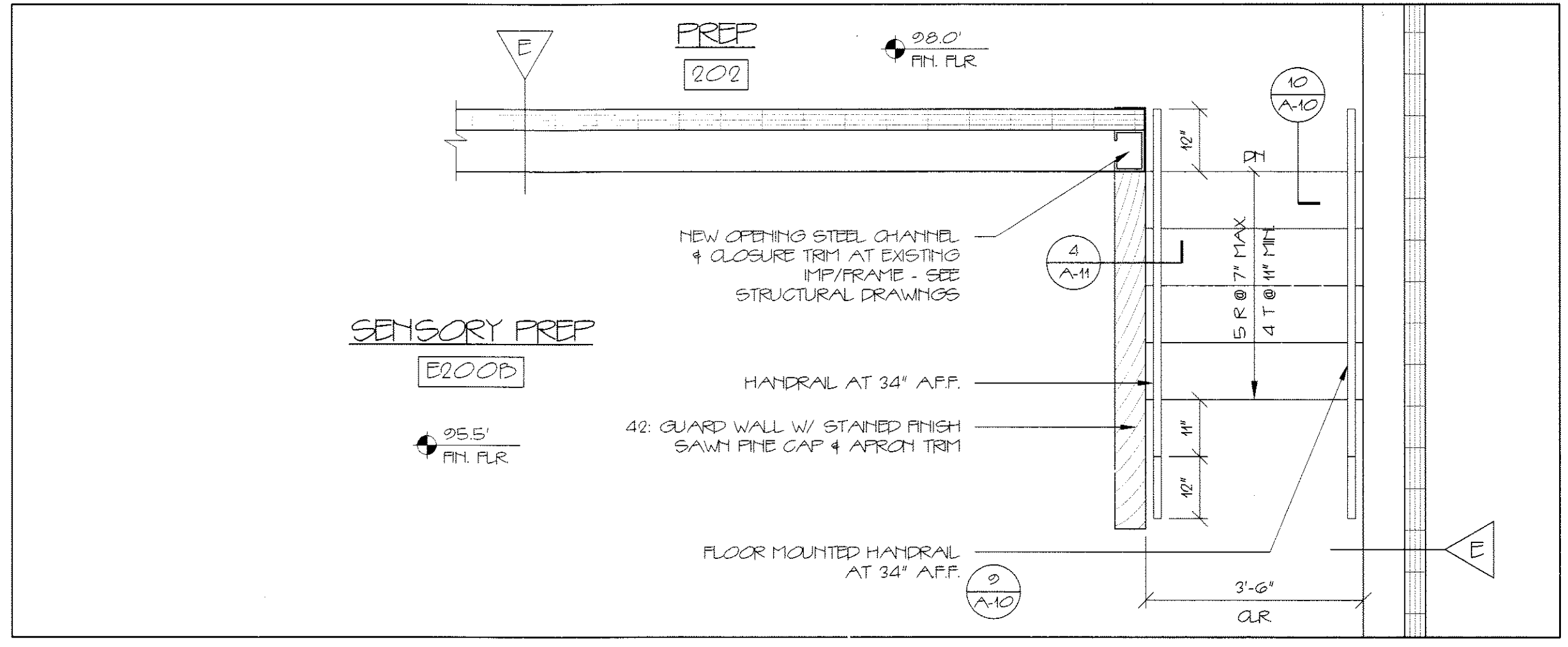
B STAR PLAN AT SENSORY PREP 1/2"=1'-0"
