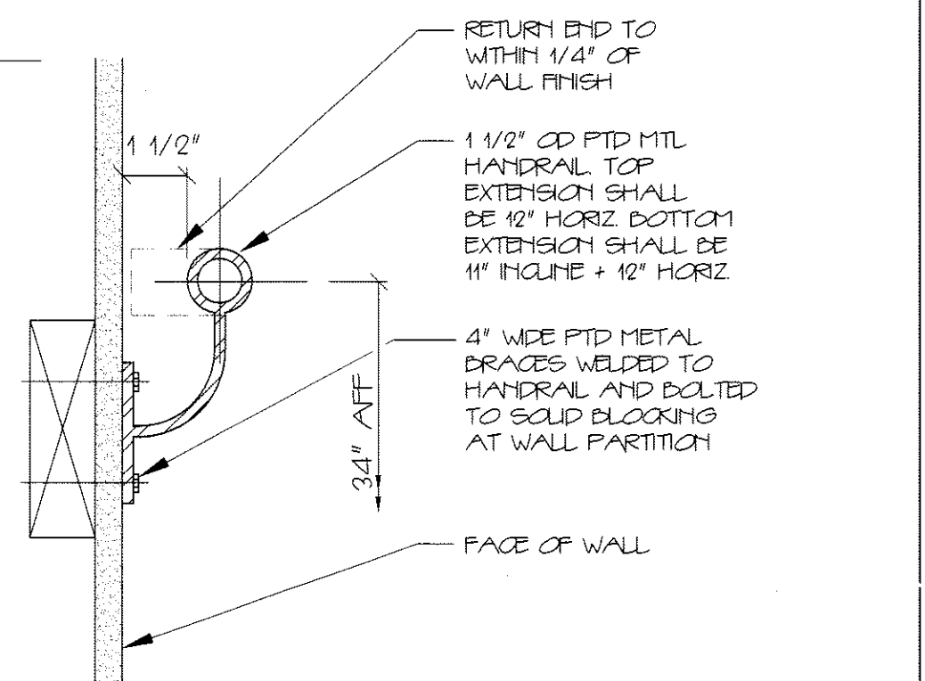
1 TYPICAL WALL HANDRAIL SECTION 3/4"=1'-0"
