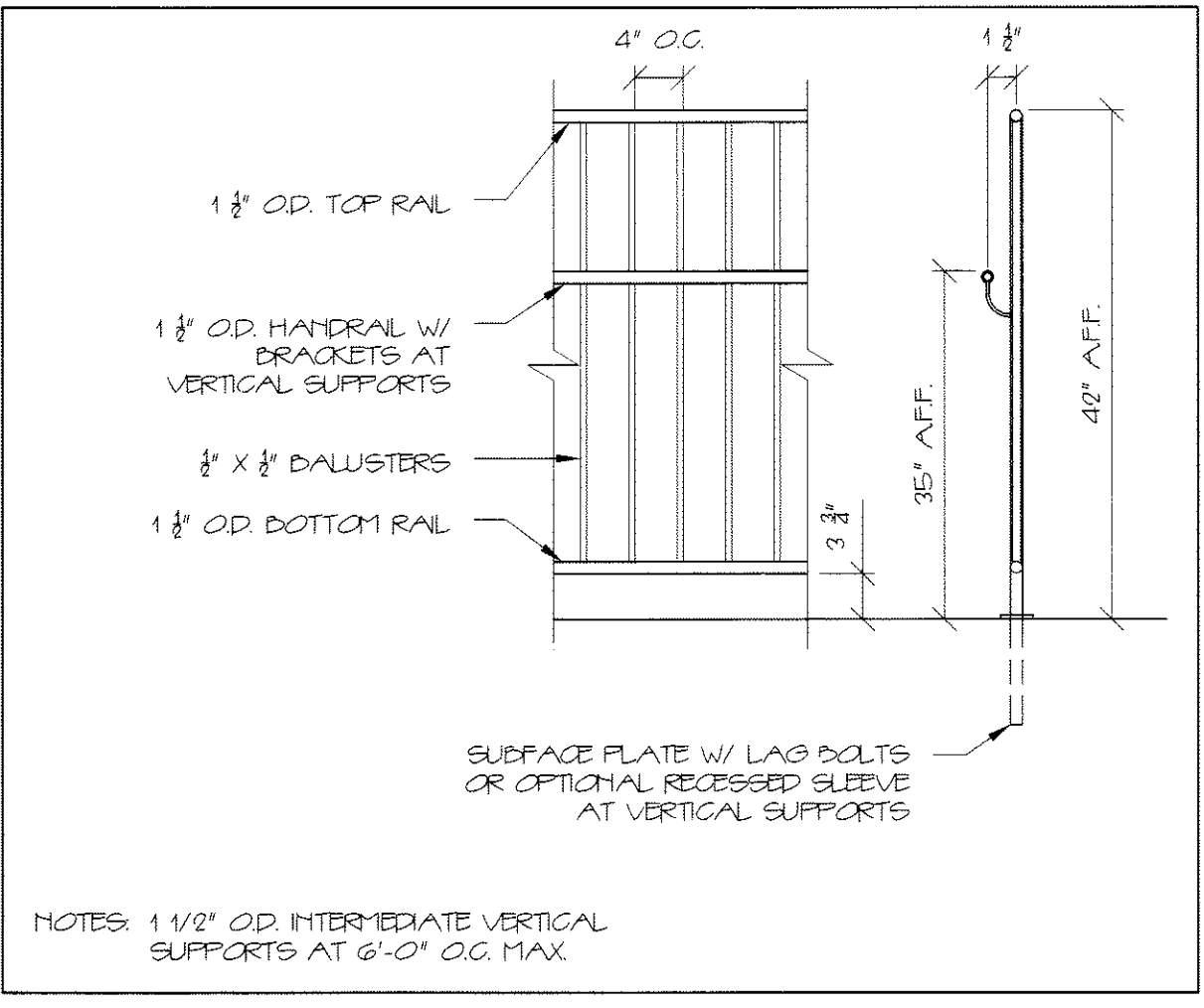
6 EXTERIOR GUARDRAIL/HANDRAIL 3/4"=1'-0"
