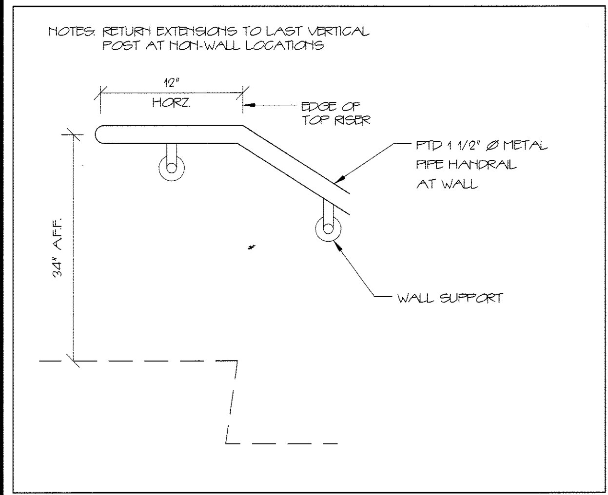
7 TYPICAL WALL HANDRAIL - BOTTOM 1 1/2"=1'-0"
