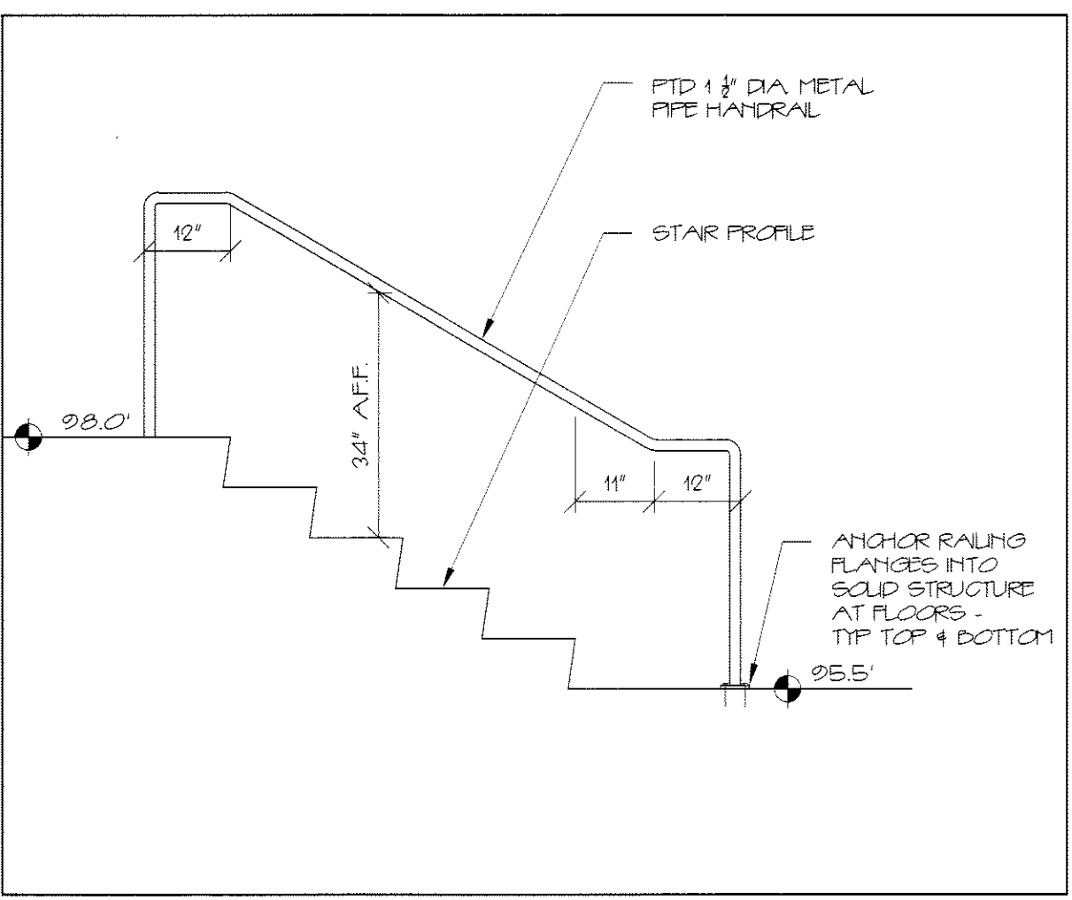
9 FLOOR MOUNTED HANDRAIL 1/2"=1'-0"
