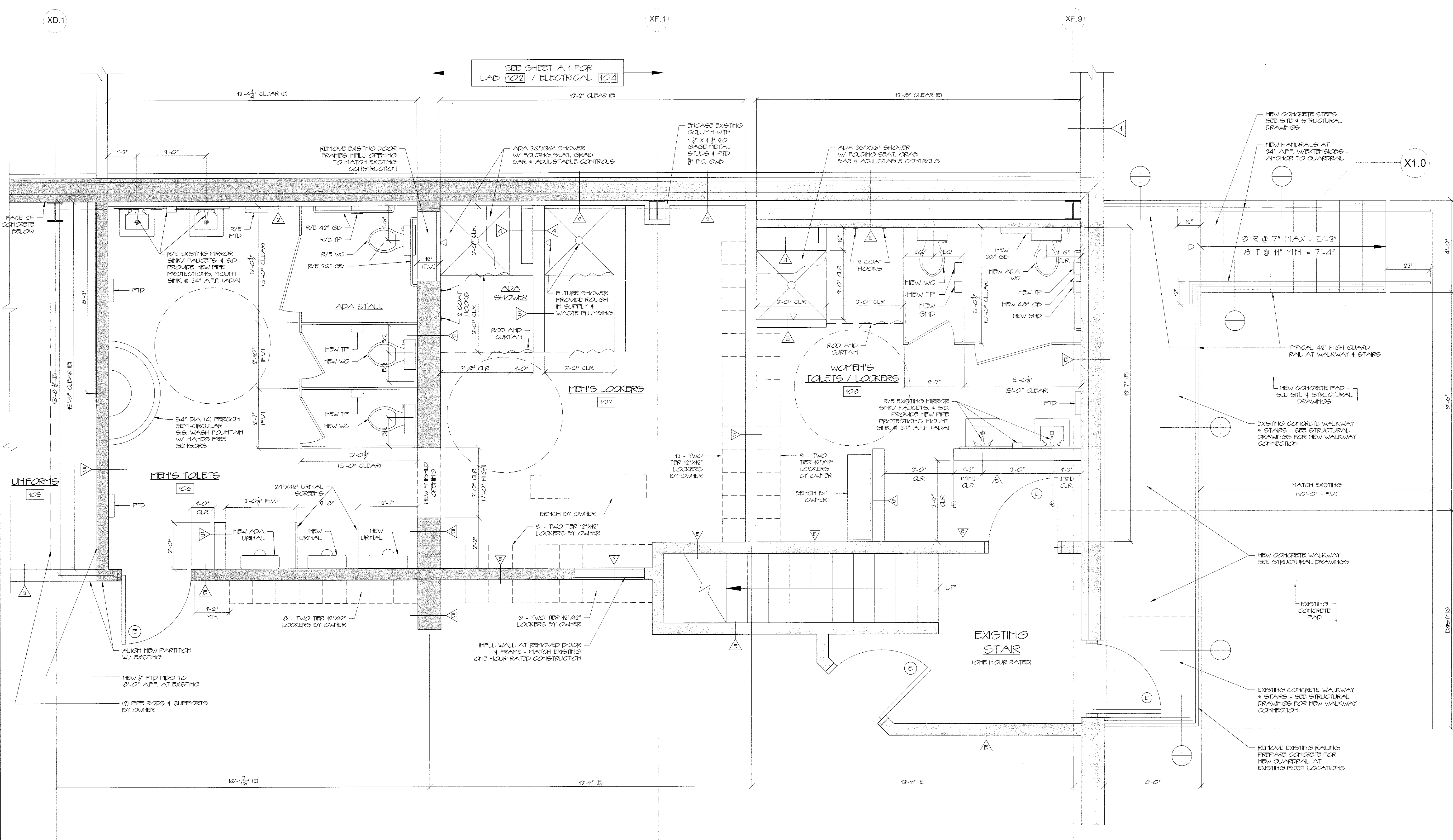
MEN'S & WOMEN'S TOILETS & LOCKERS AREA SCALE: 1/2" = 1'-0"
