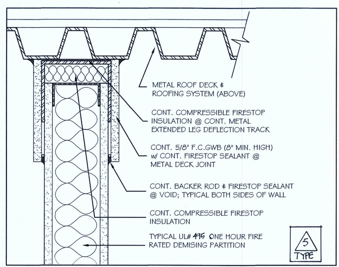
② TYP. 1 HR RATED PARTITION @ DEFLECTION TRACK 3"=1'-0"
