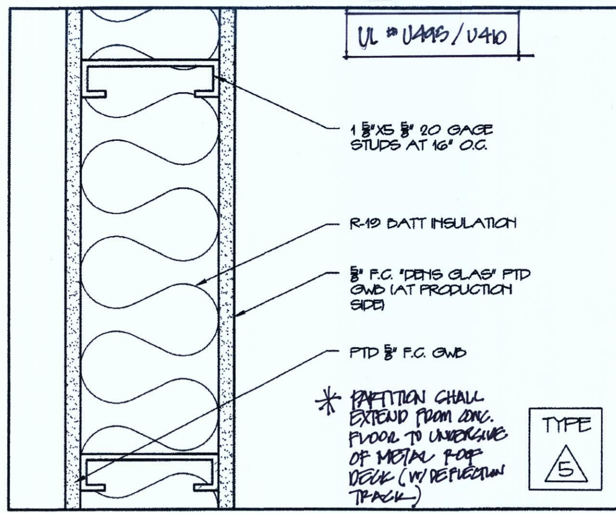
① ONE HOUR RATED PARTITION 3"=1'-0"
