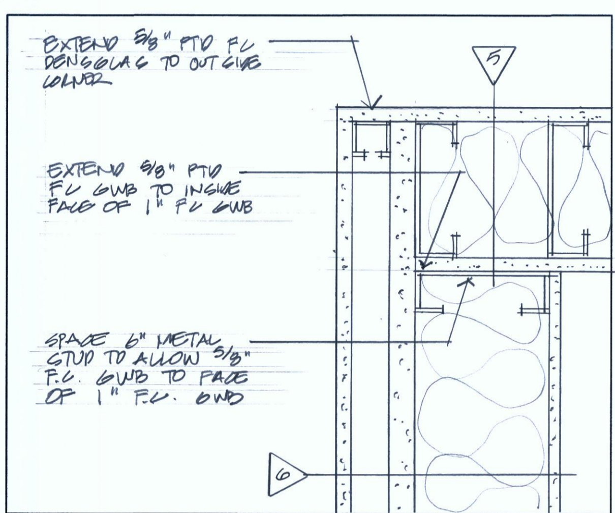
⑥ PLAN DETAIL AT 1 HR RATED PARTITIONS 3"=1'-0"
