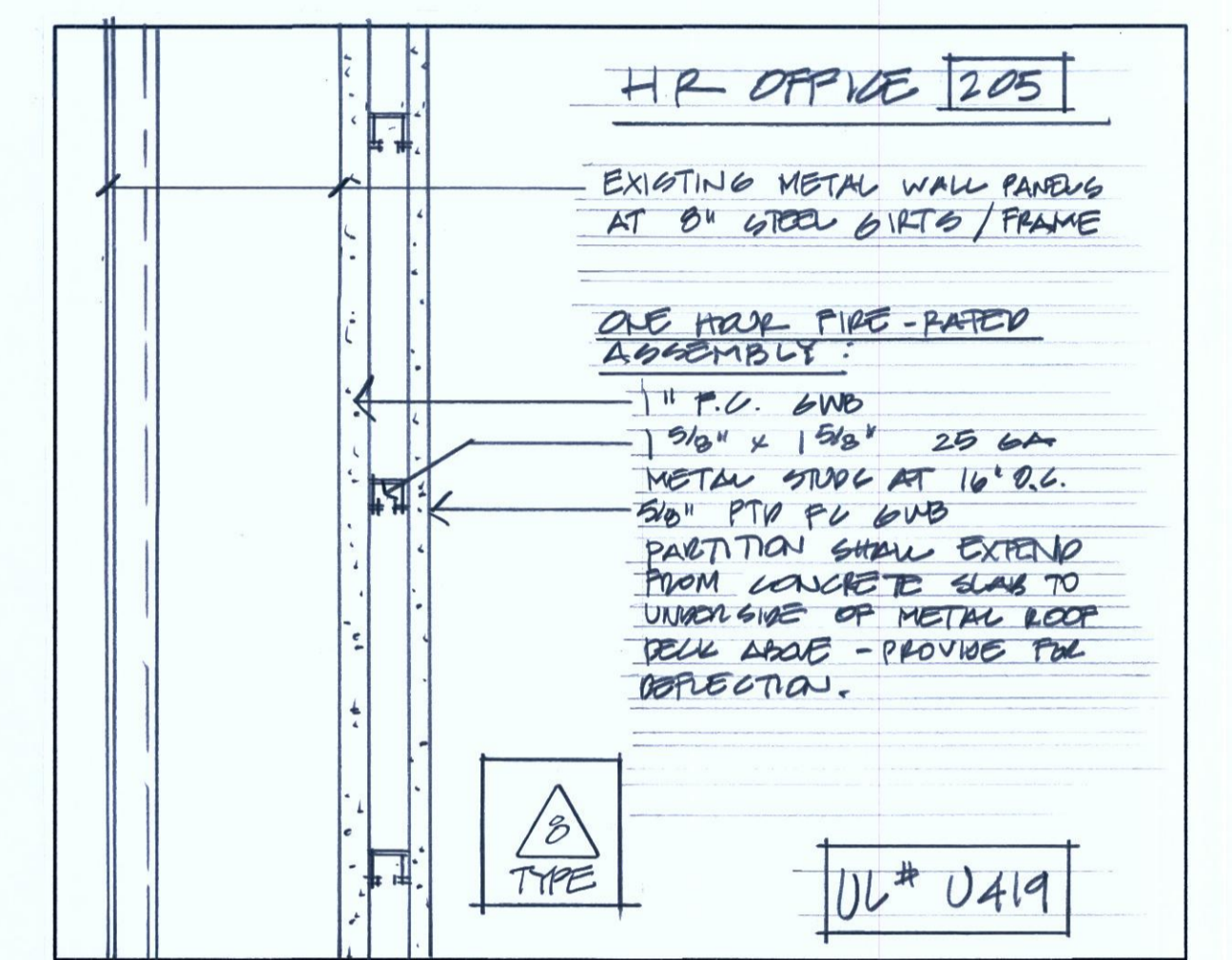
⑤ ONE HOUR FIRE RATED PARTITION 3"=1'-0"
