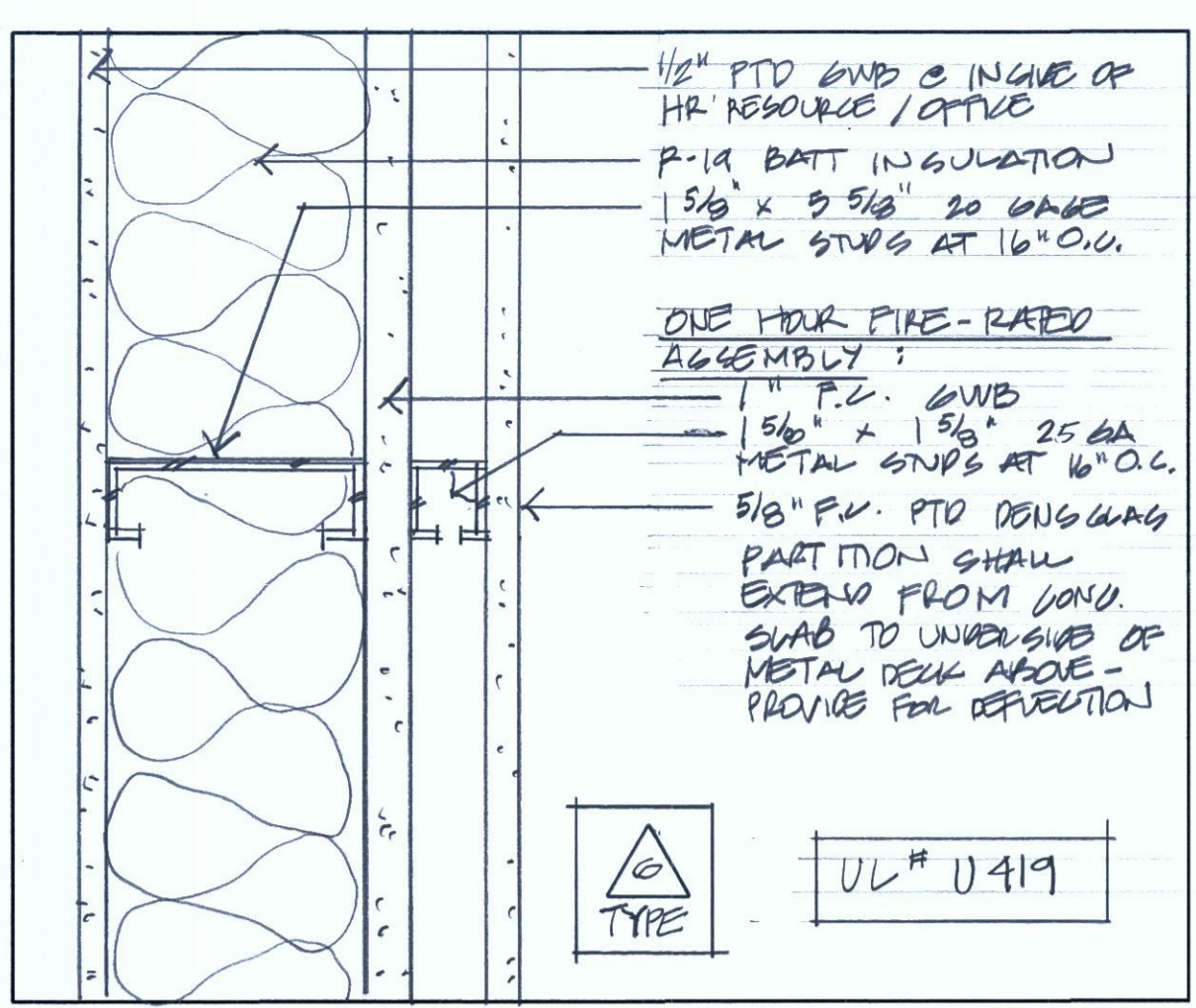
③ ONE HOUR FIRE RATED PARTITION 3"=1'-0"
