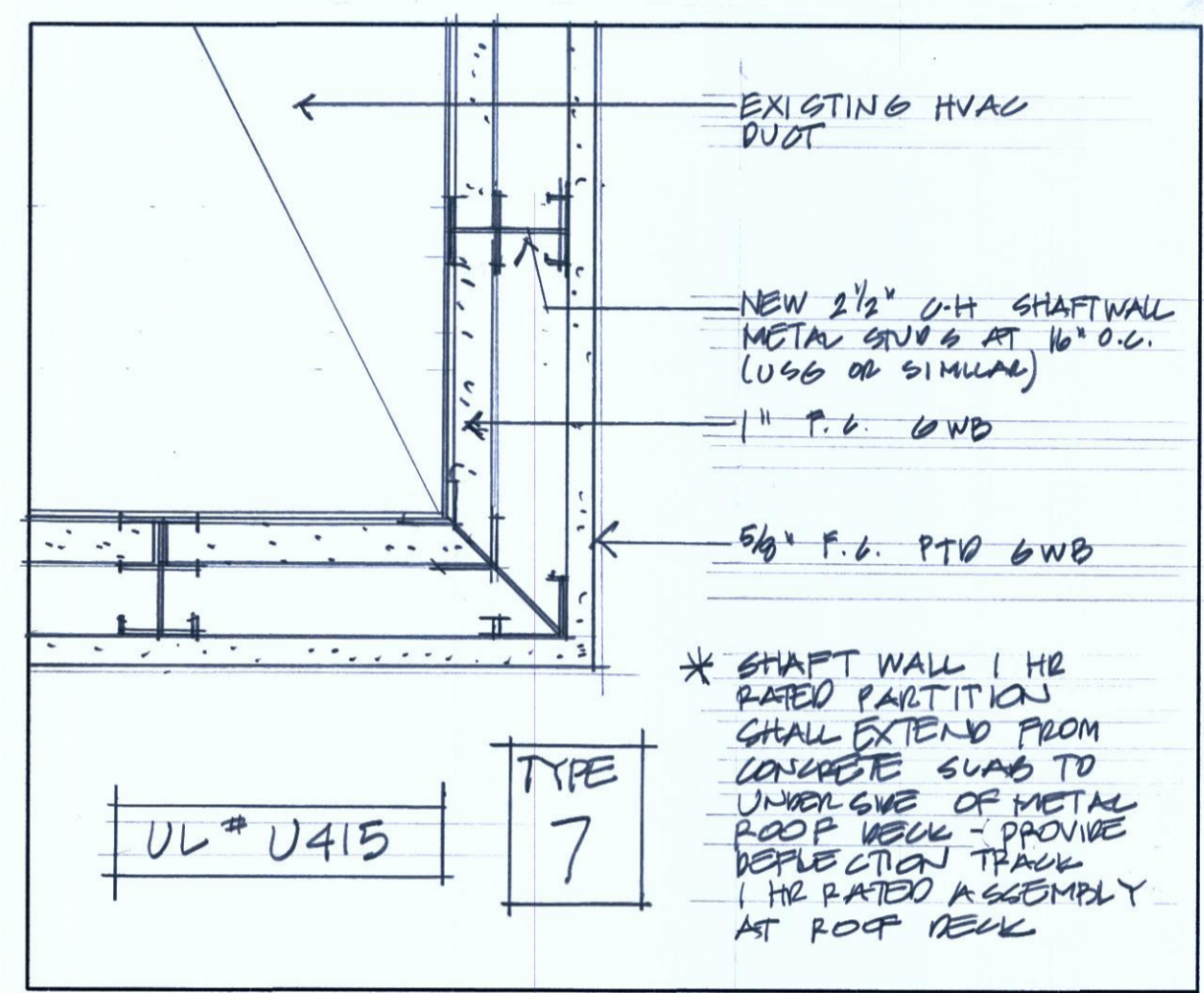
④ ONE HOUR RATED SHAFT WALL 3"=1'-0"
