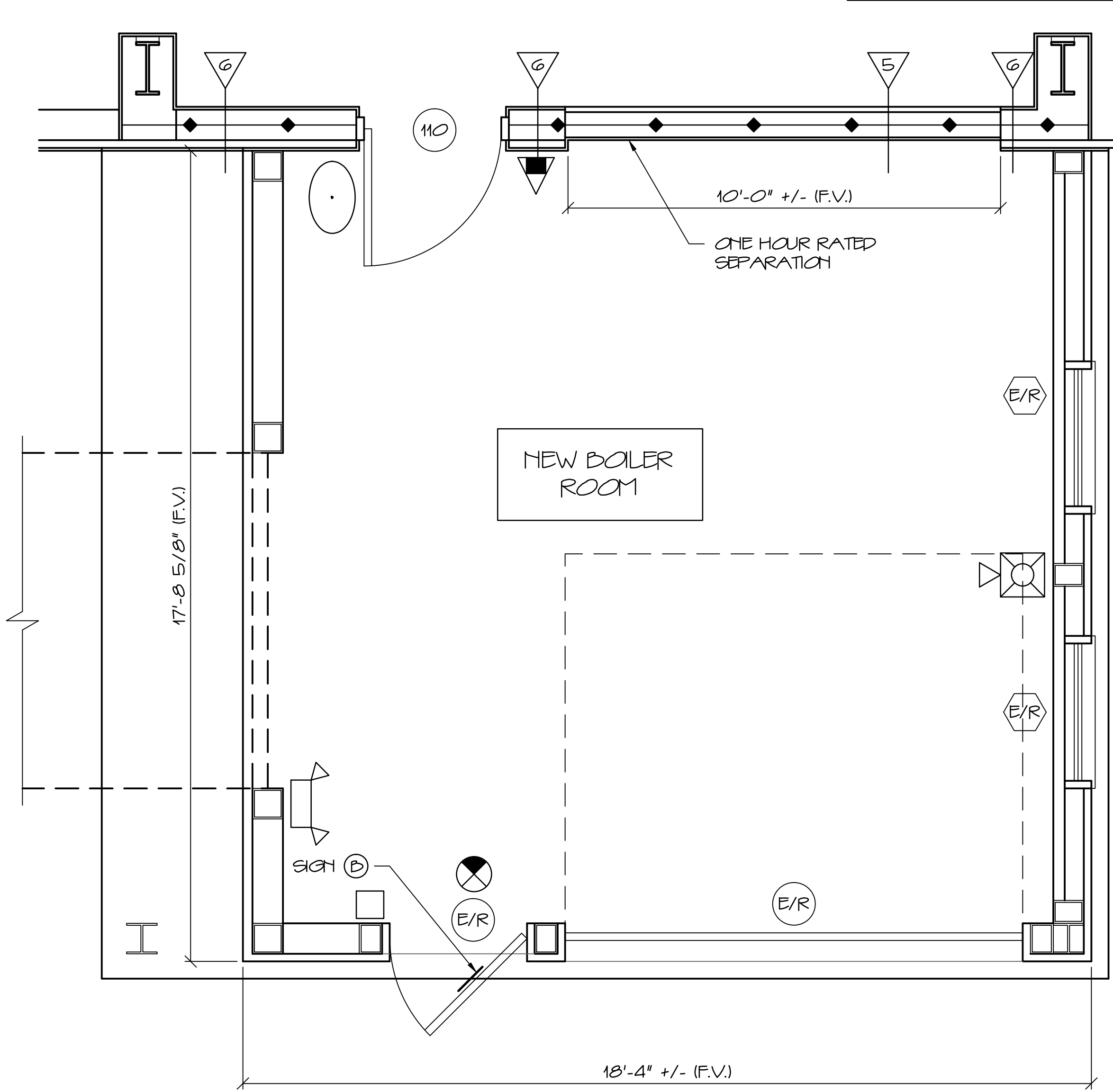
CODE COMPLIANCE FLOOR PLAN 1/2" = 1'-0"
