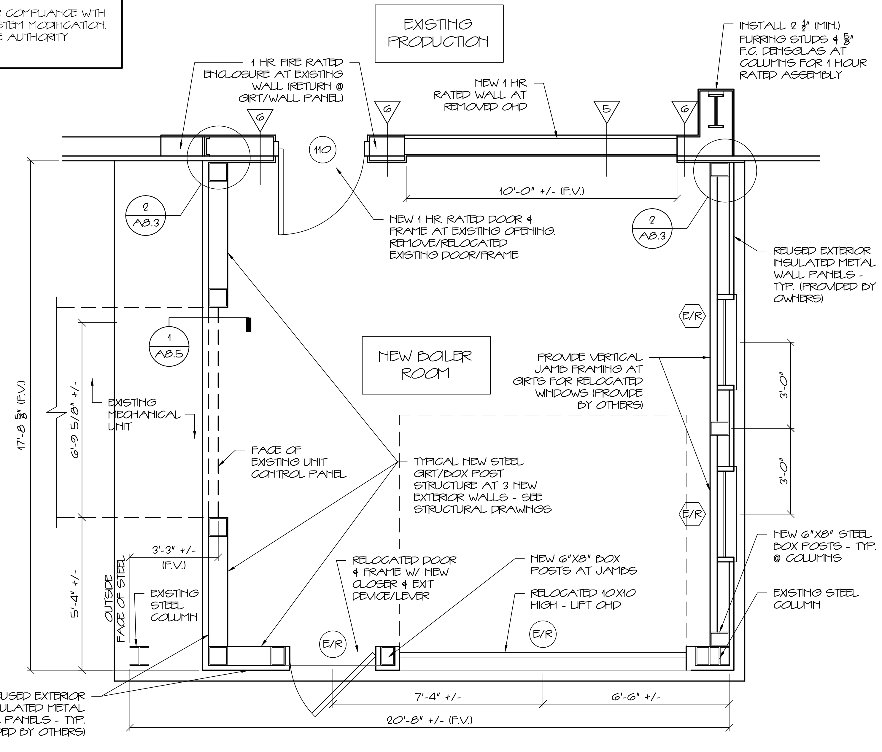
FLOOR PLAN 1/2" = 1'-0"
