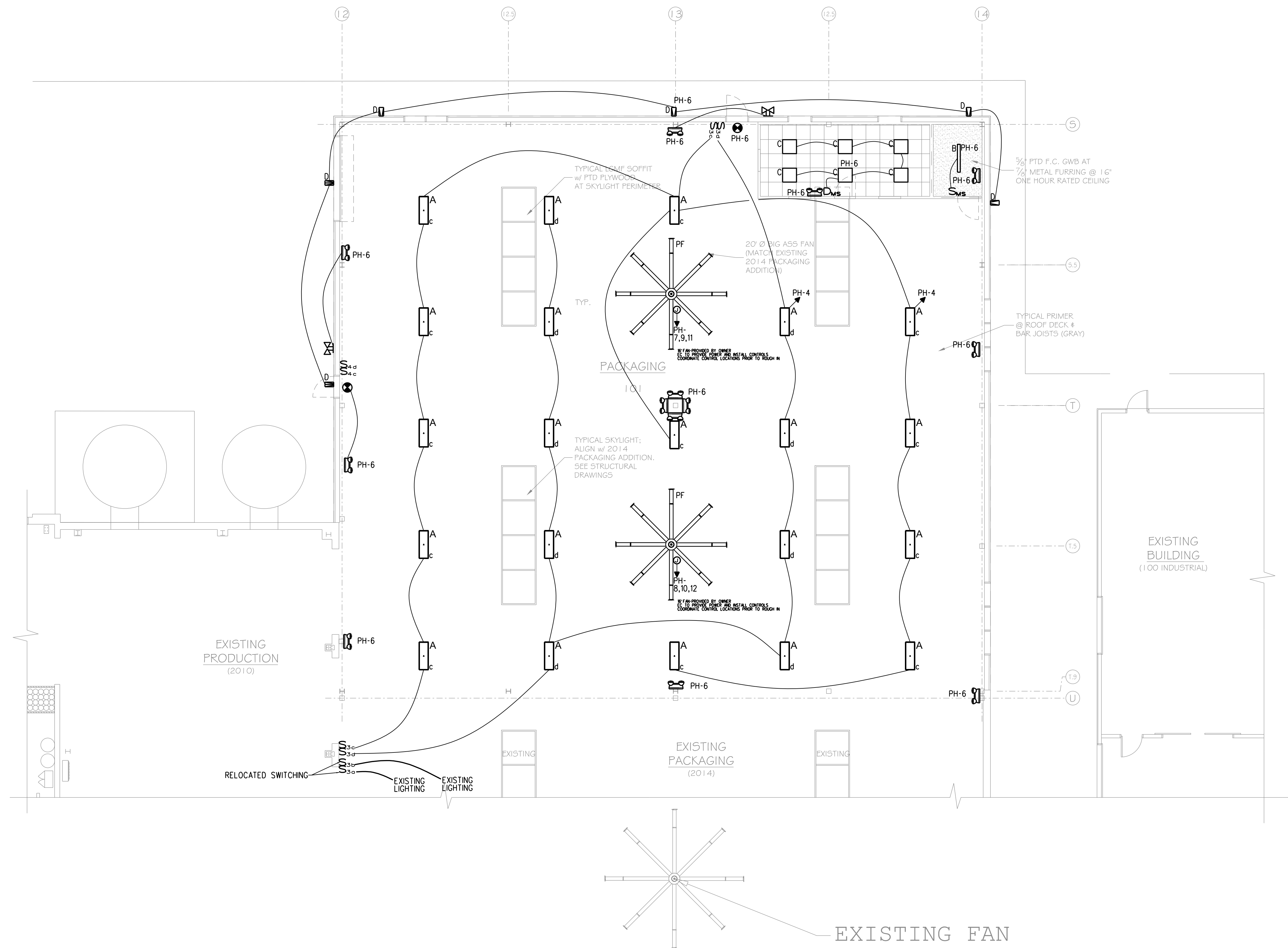
ADDITION LIGHTING PLAN SCALE: 1/8" = 1'-0"
