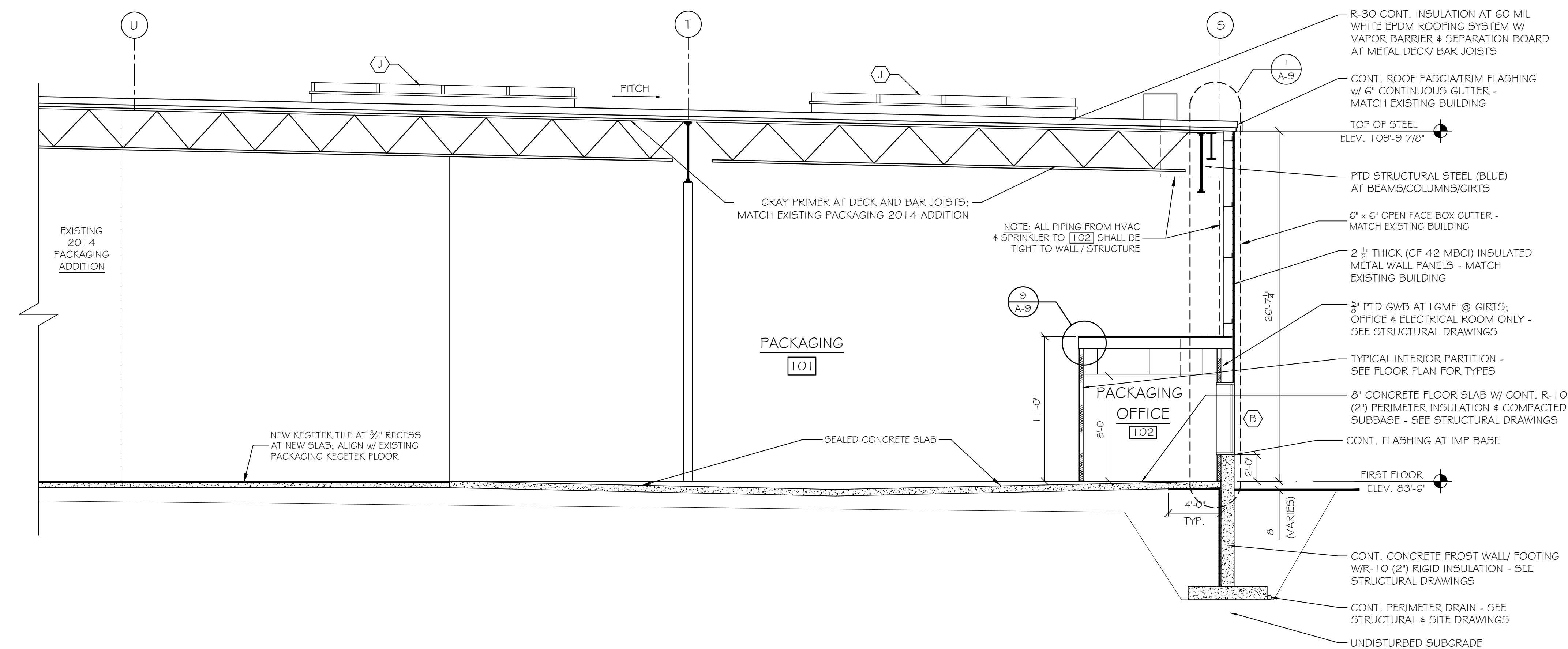
B BUILDING SECTION B SCALE: 3/16" = 1'-0"
