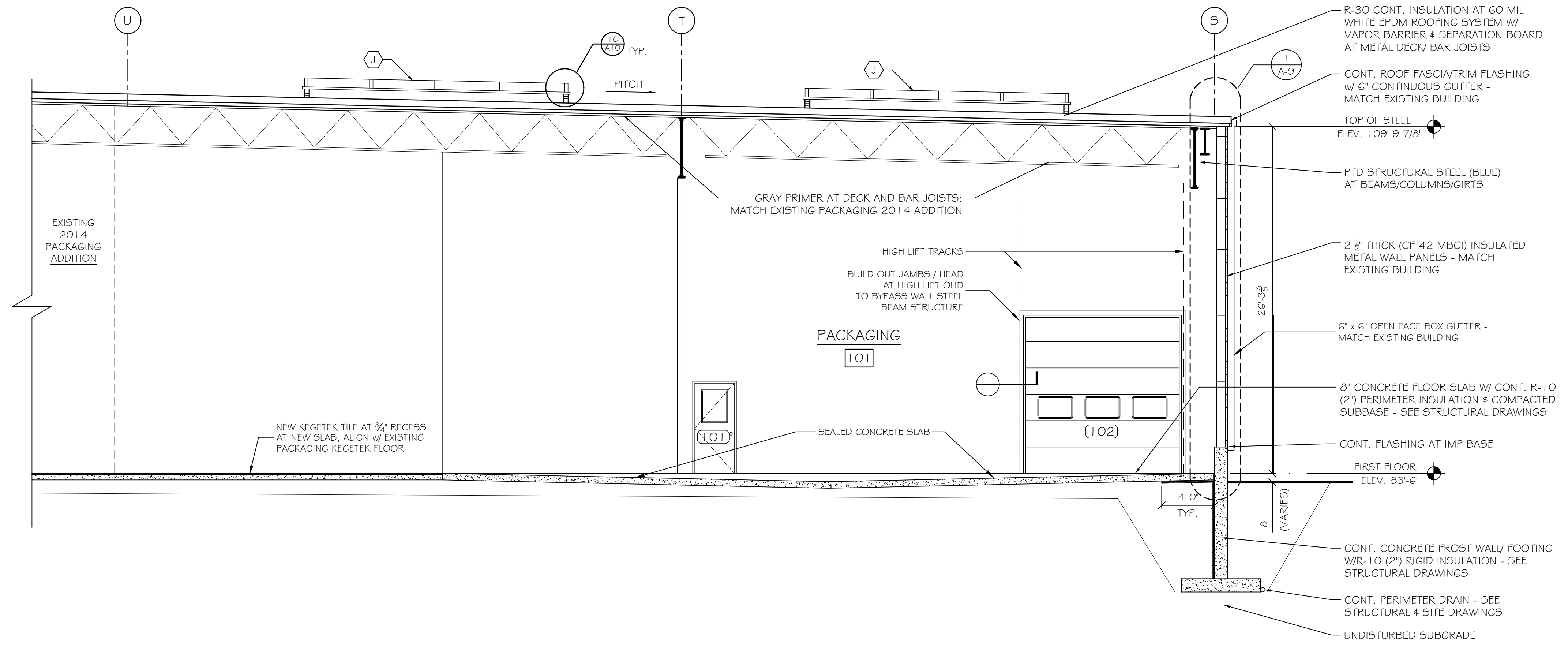
A BUILDING SECTION A SCALE: 3/16" = 1'-0"
