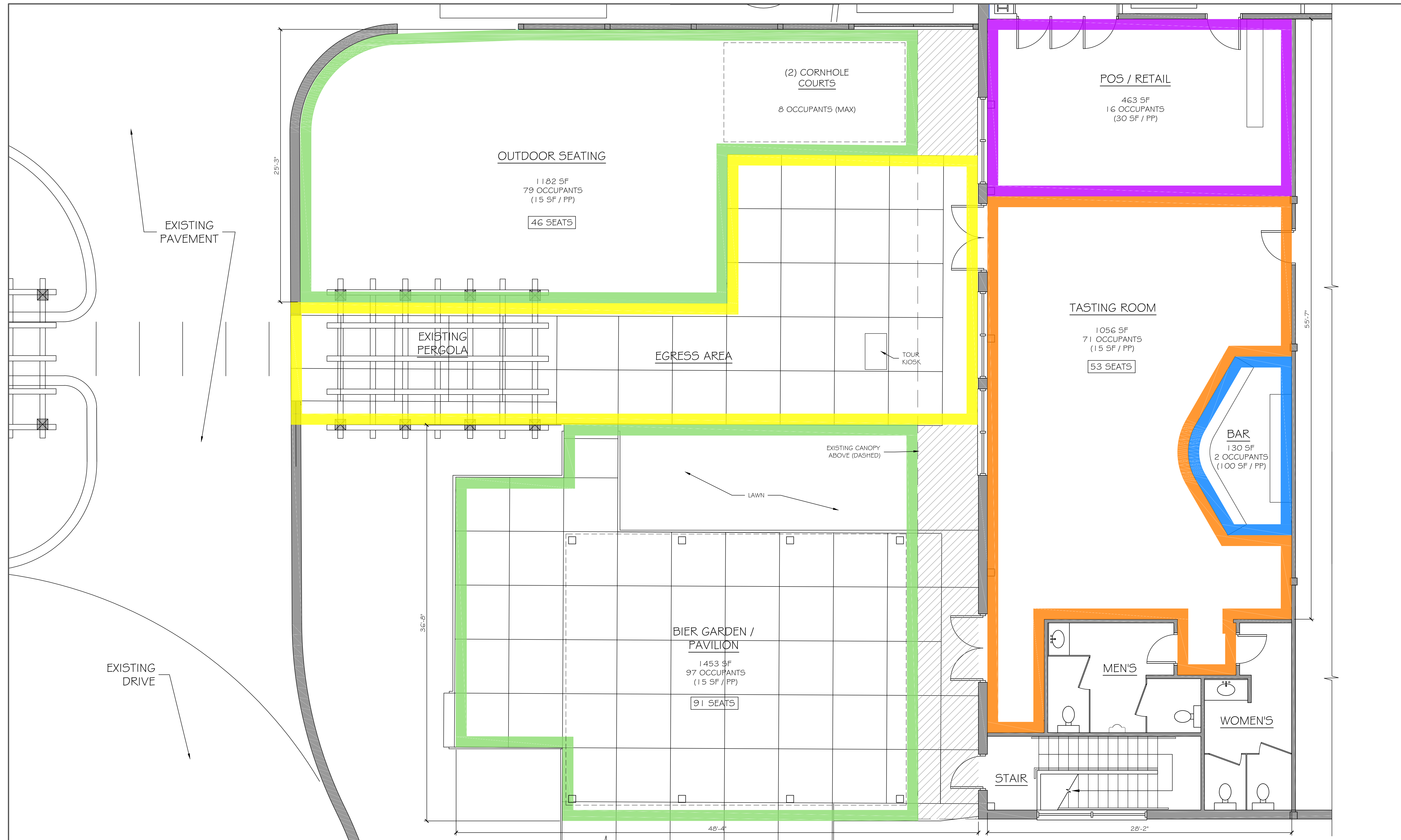
TASTING ROOM / OUTDOOR SEATING OCCUPANCY PLAN SCALE: 1/4" = 1'-0"
