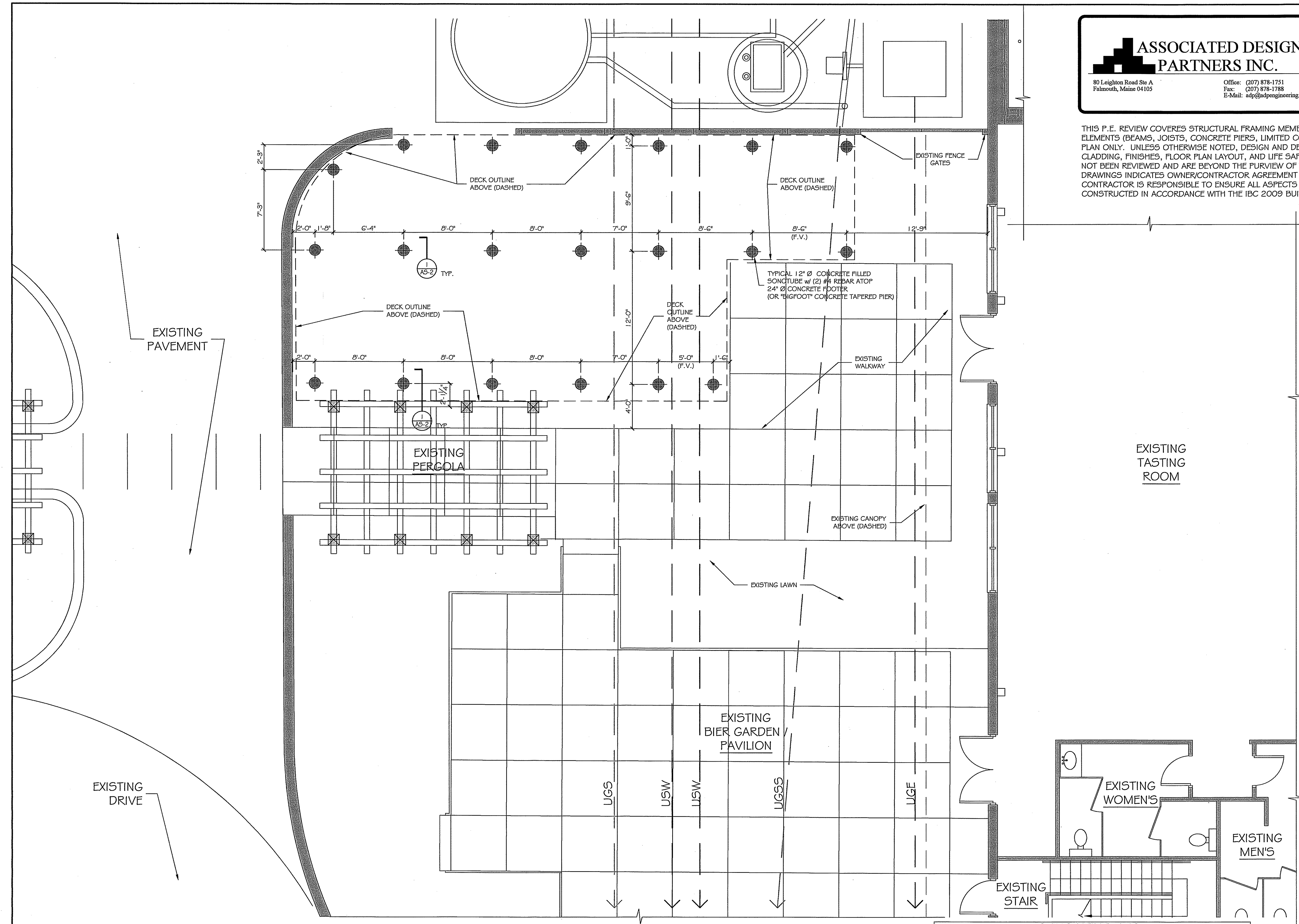
NEW DECK FOOTING PLAN SCALE: 1/4" = 1'-0"
