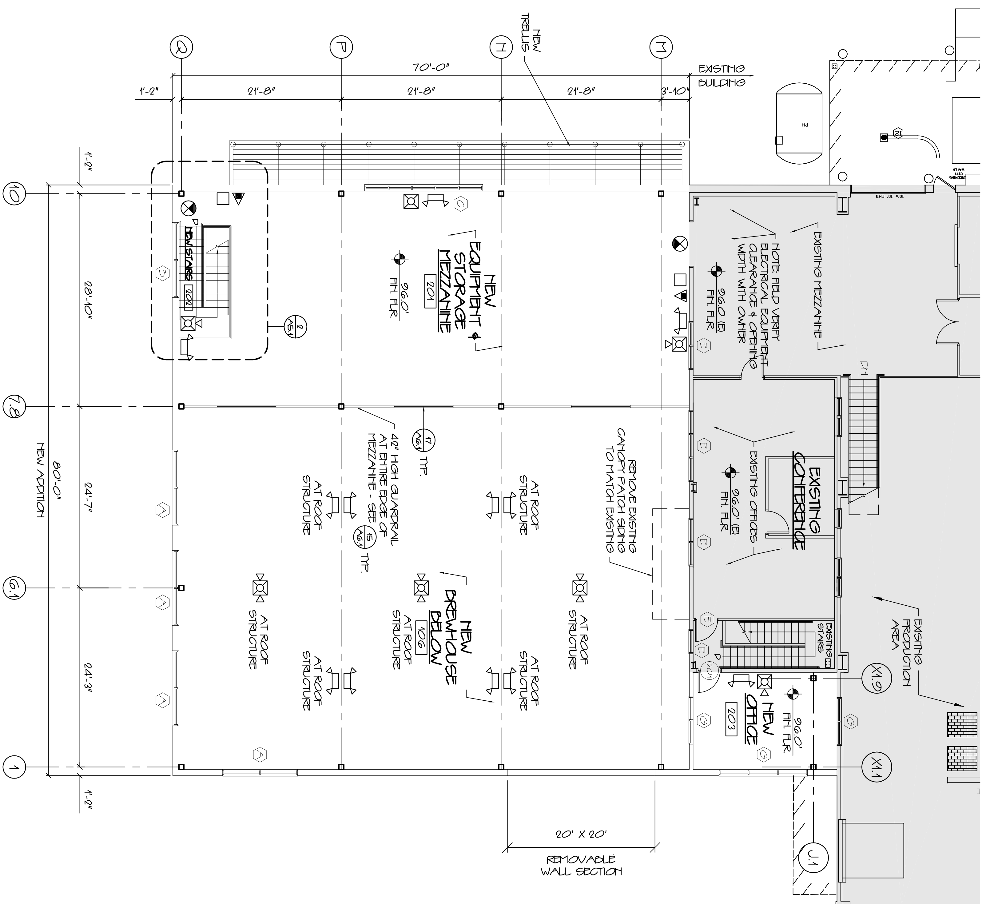
2 SECOND FLOOR NEW ADDITION CODE COMPLIANCE PLAN SCALE 1/8" = 1'-0"
