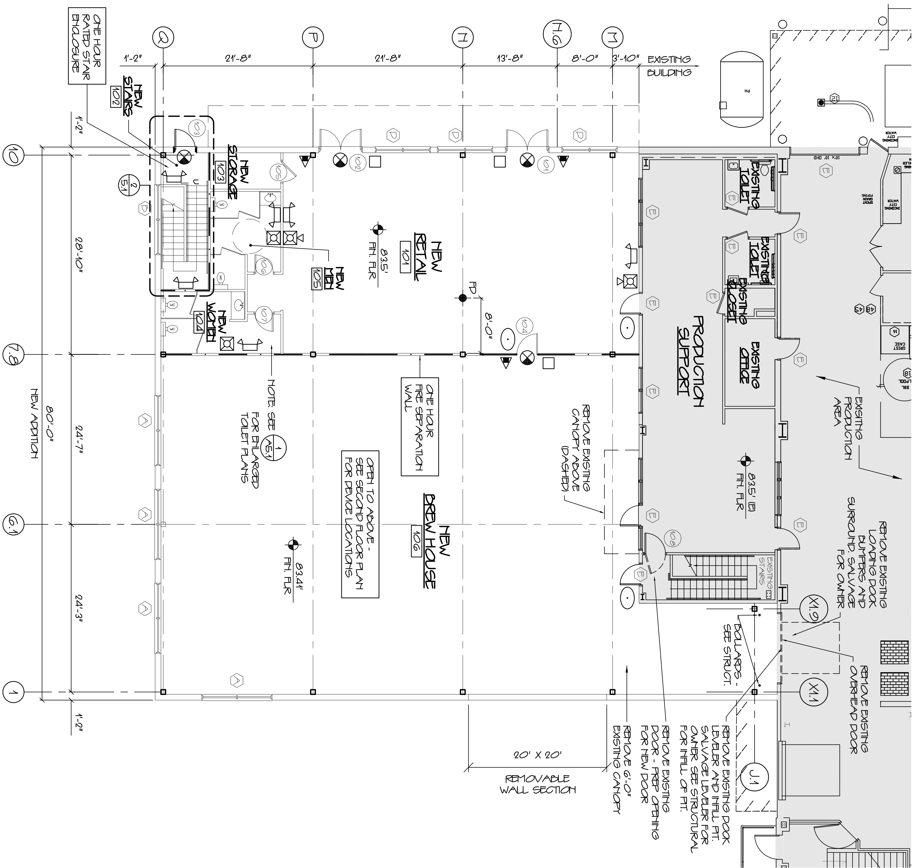
1 FIRST FLOOR NEW ADDITION CODE COMPLIANCE PLANS SCALE 1/8" = 1'-0"
