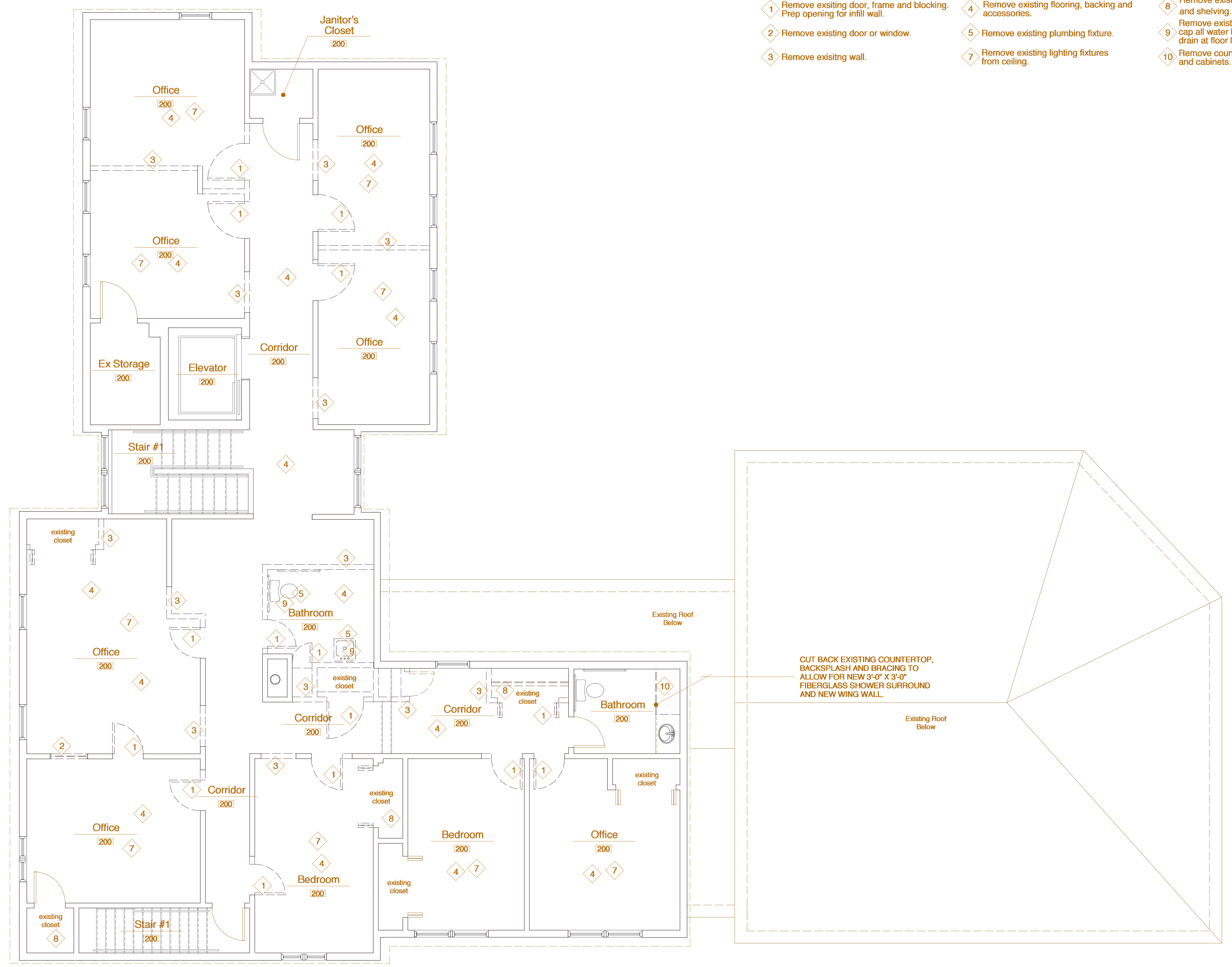
10 Second Floor Demolition Plan 0 4 12 24
