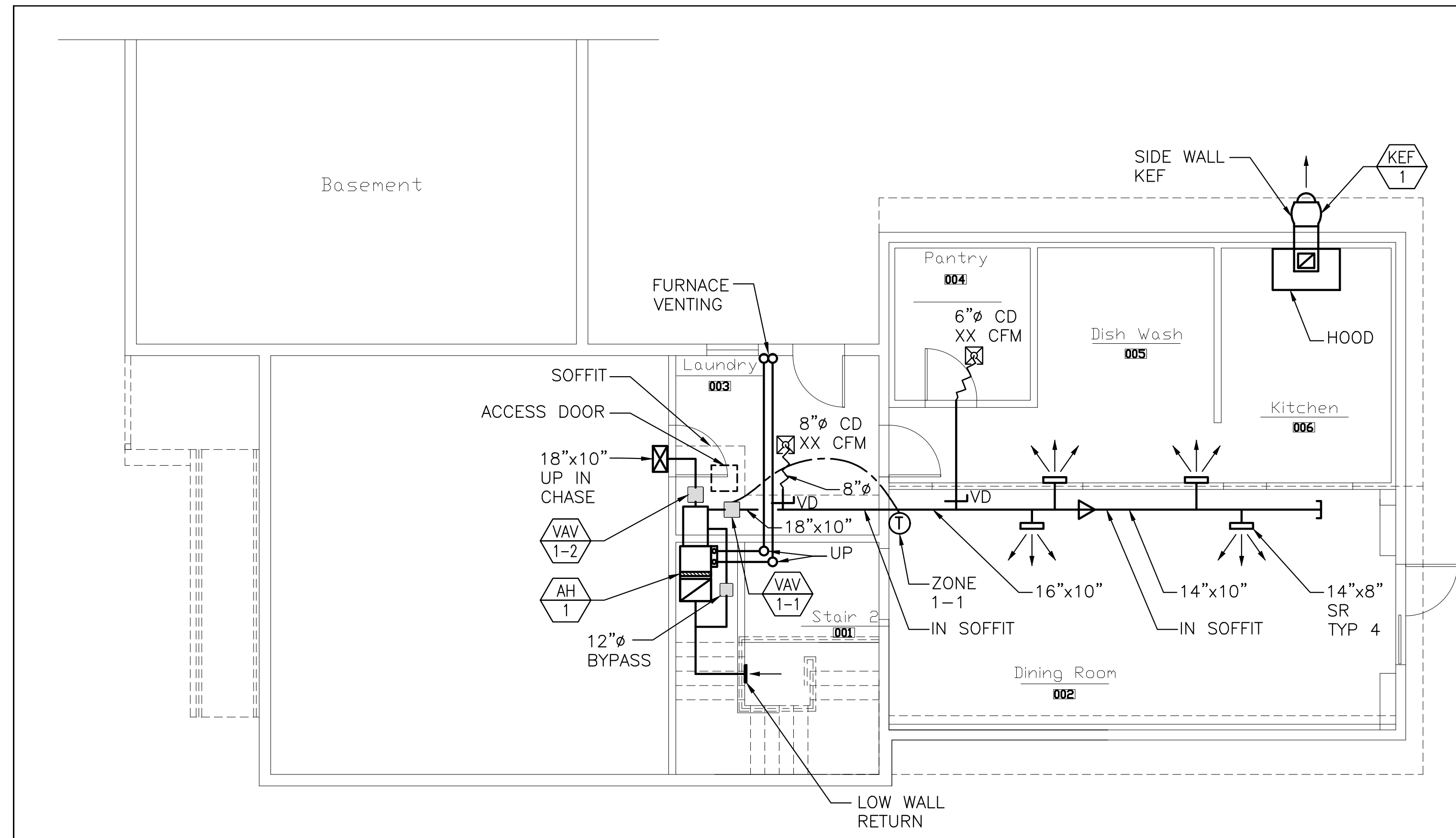
Partial Ground Floor Plan
