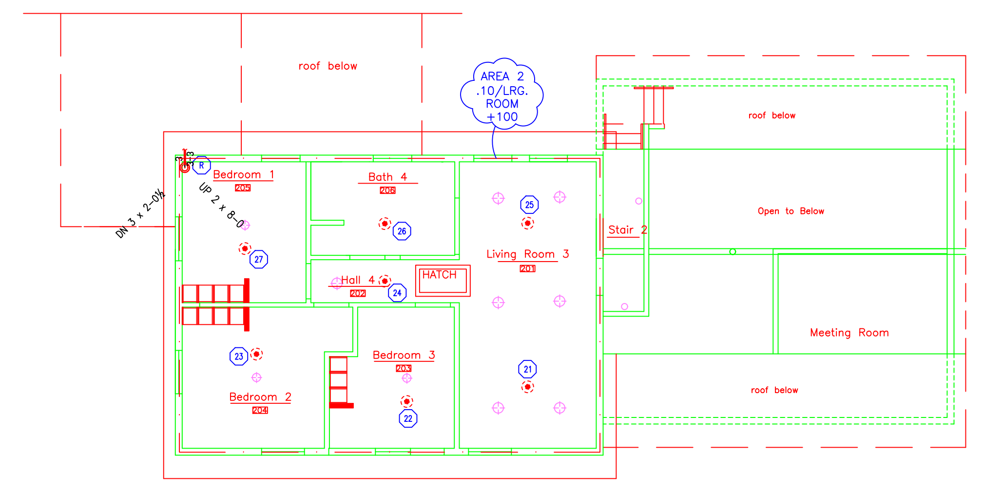
PARTIAL THIRD FLOOR SPRINKLER PLAN SCALE: 1/8" = 1'-0" FINISH FLOOR ELEV. 117.67'
