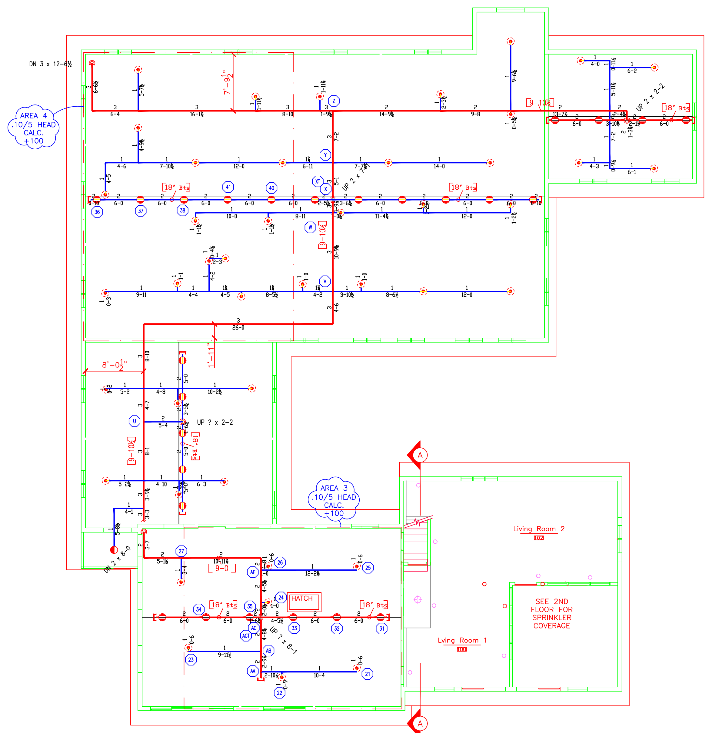
ROOF SPRINKLER PLAN SCALE: 1/8" = 1'-0"
