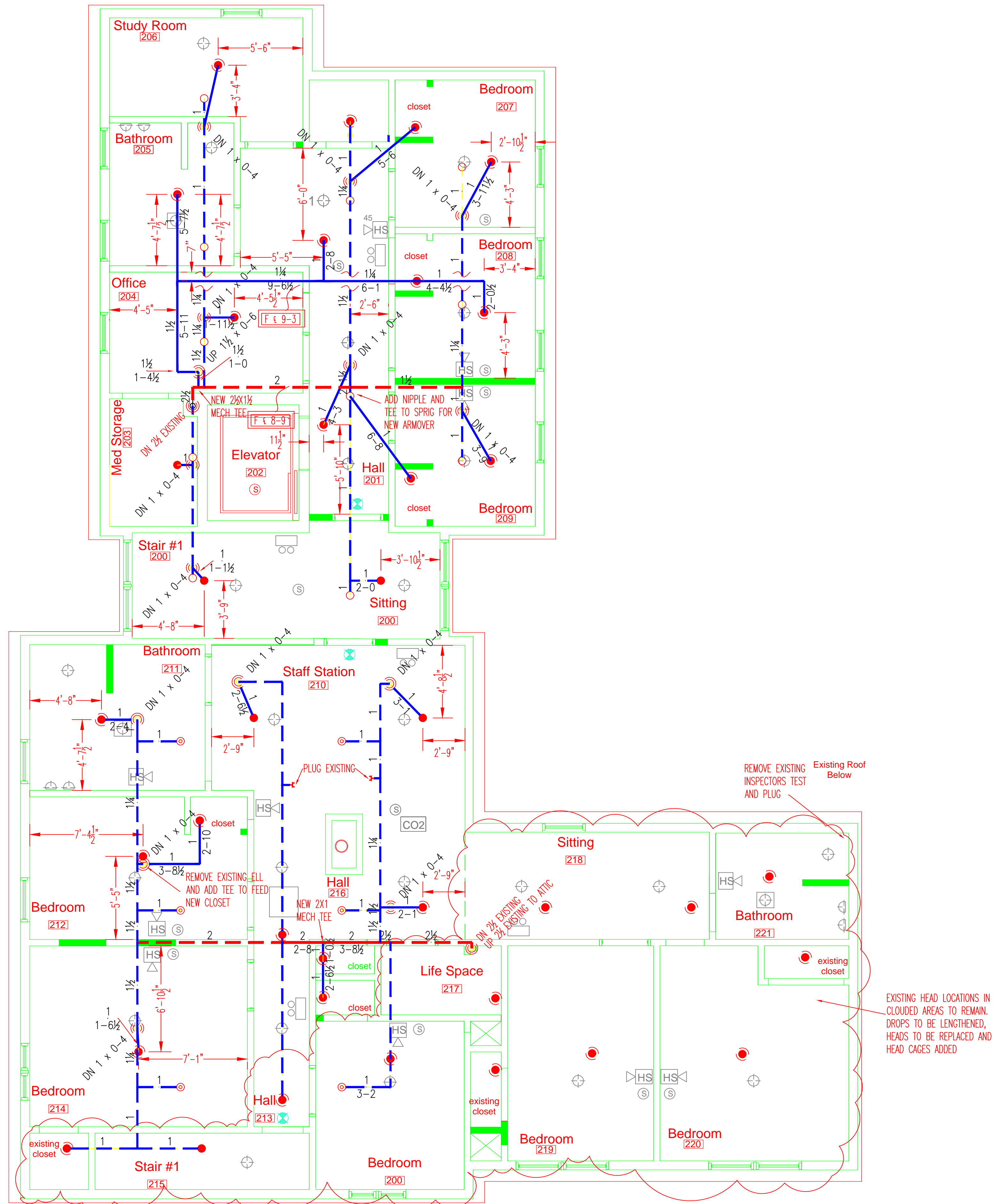
SECOND FLOOR LAYOUT SCALE 1/4"=1'-0"
