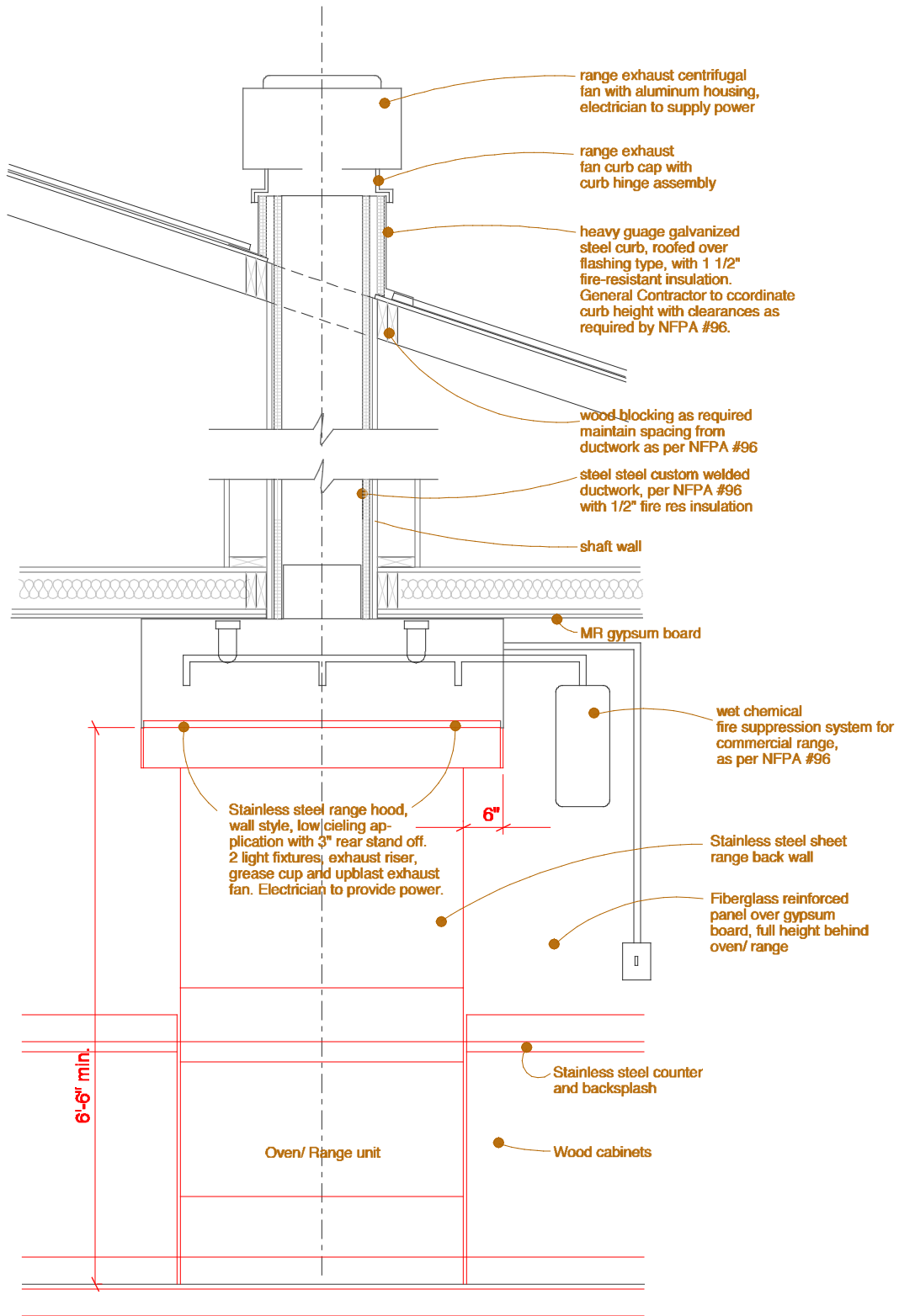
10 Section Detail
