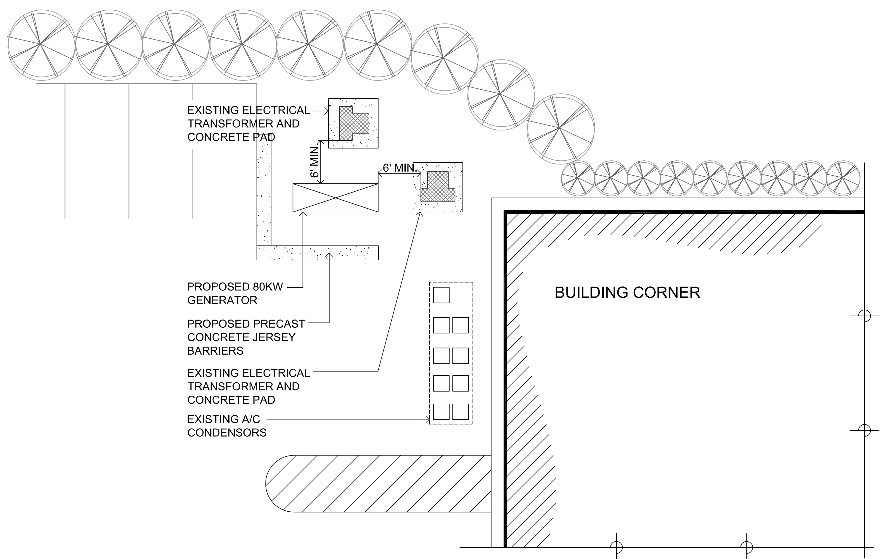
ENLARGED PLAN
