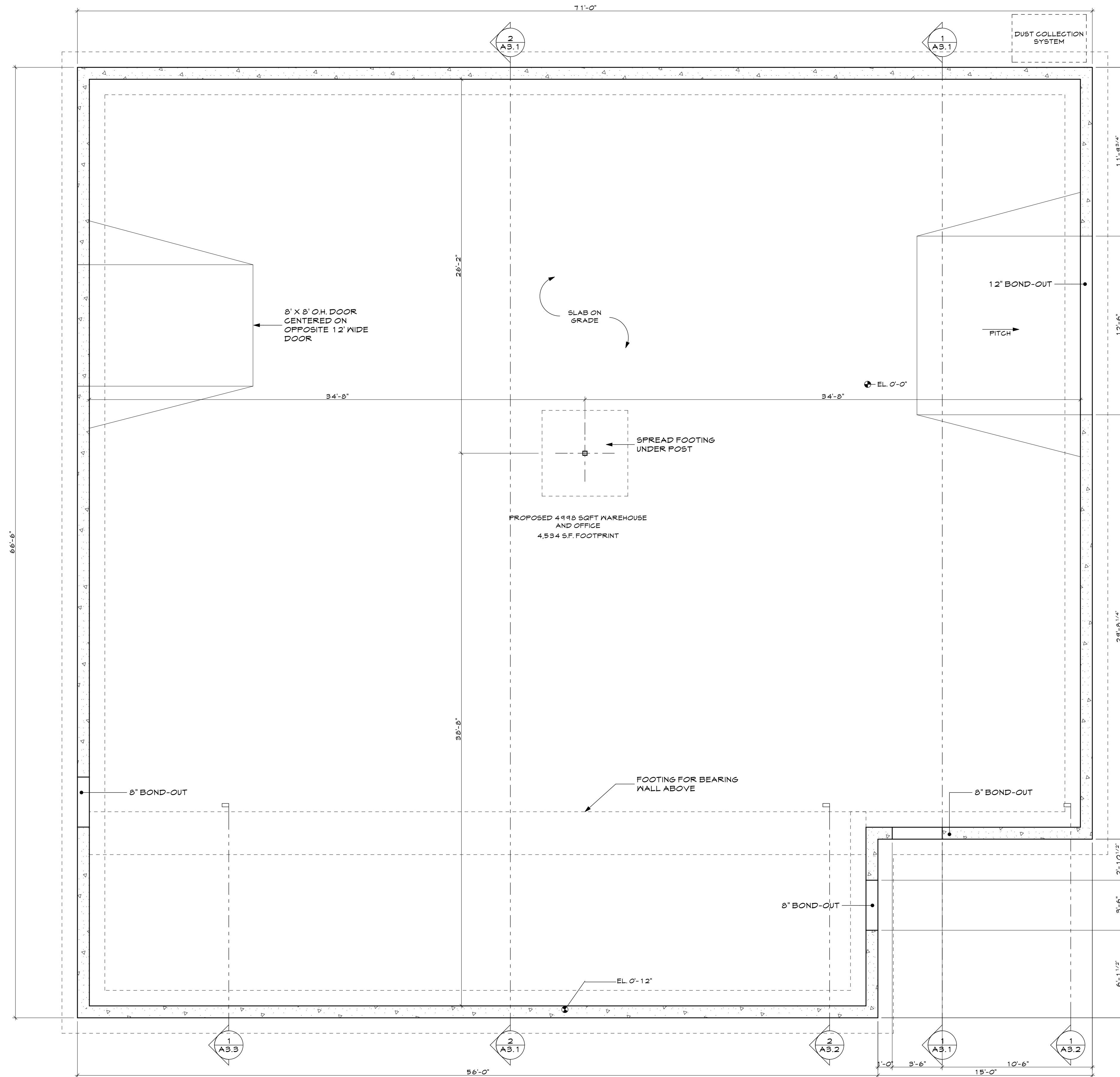
1 FOUNDATION PLAN A1.1 SCALE: 1/4" = 1'-0"
