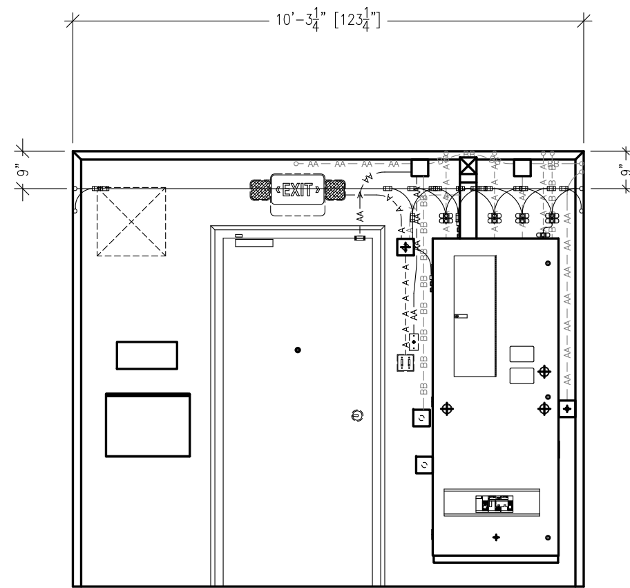
ELEVATION "D"
