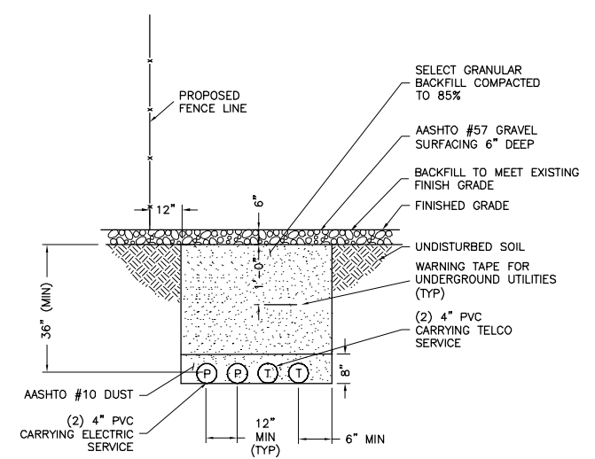
NOTE: 1. EXCAVATE EXISTING SUBGRADE AS REQUIRED TO INSTALL CONDUITS IN ACCORDANCE WITH OSHA AND ALL APPLICABLE CODES. 2 TYPICAL TRENCH DETAIL E-1 NTS
