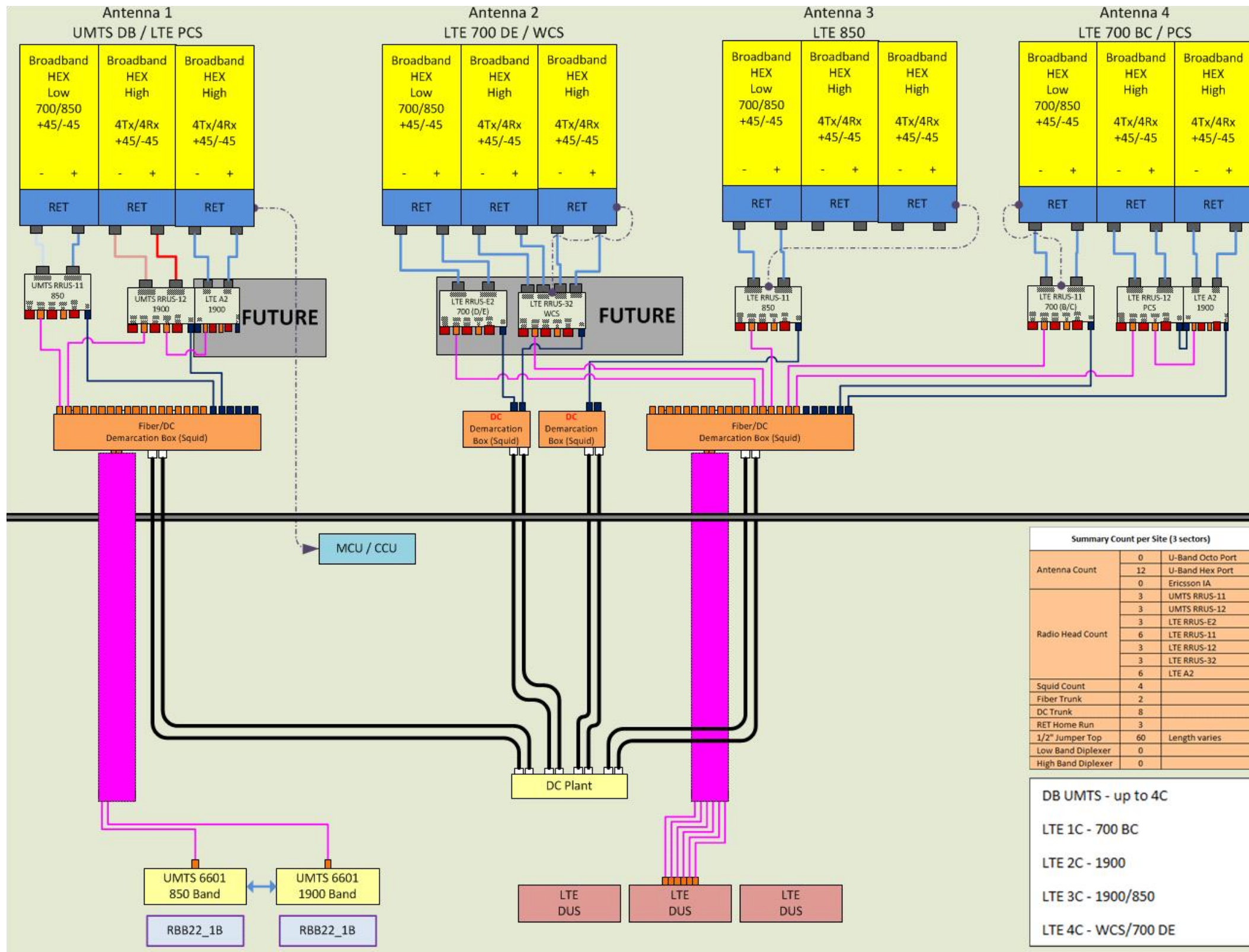
1 RF PLUMBING DIAGRAM A-3 NTS
