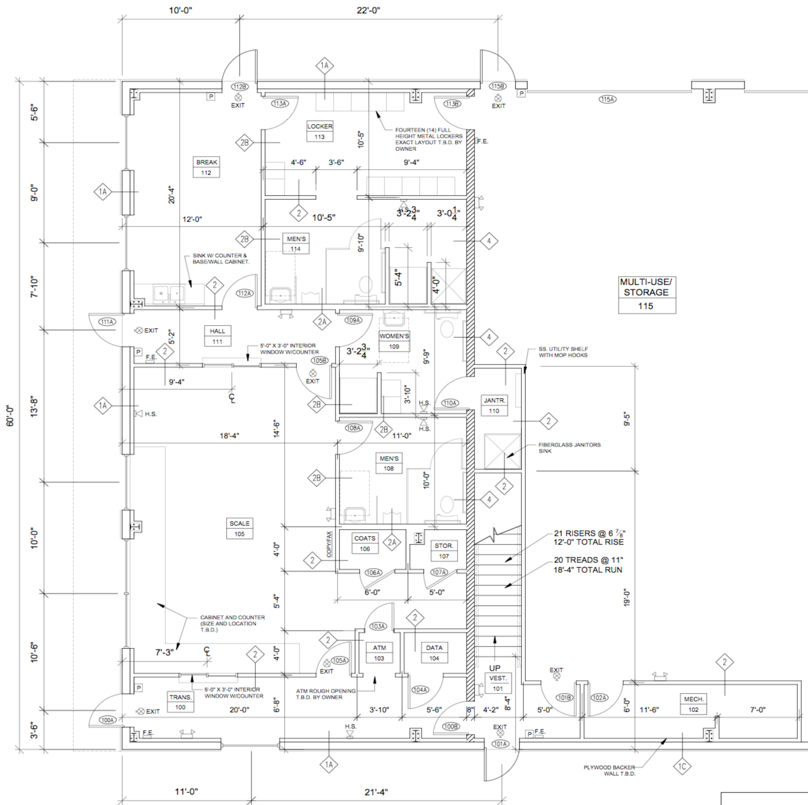
FIRST FLOOR OFFICE PLAN SCALE: 1/4"=1'-0"
