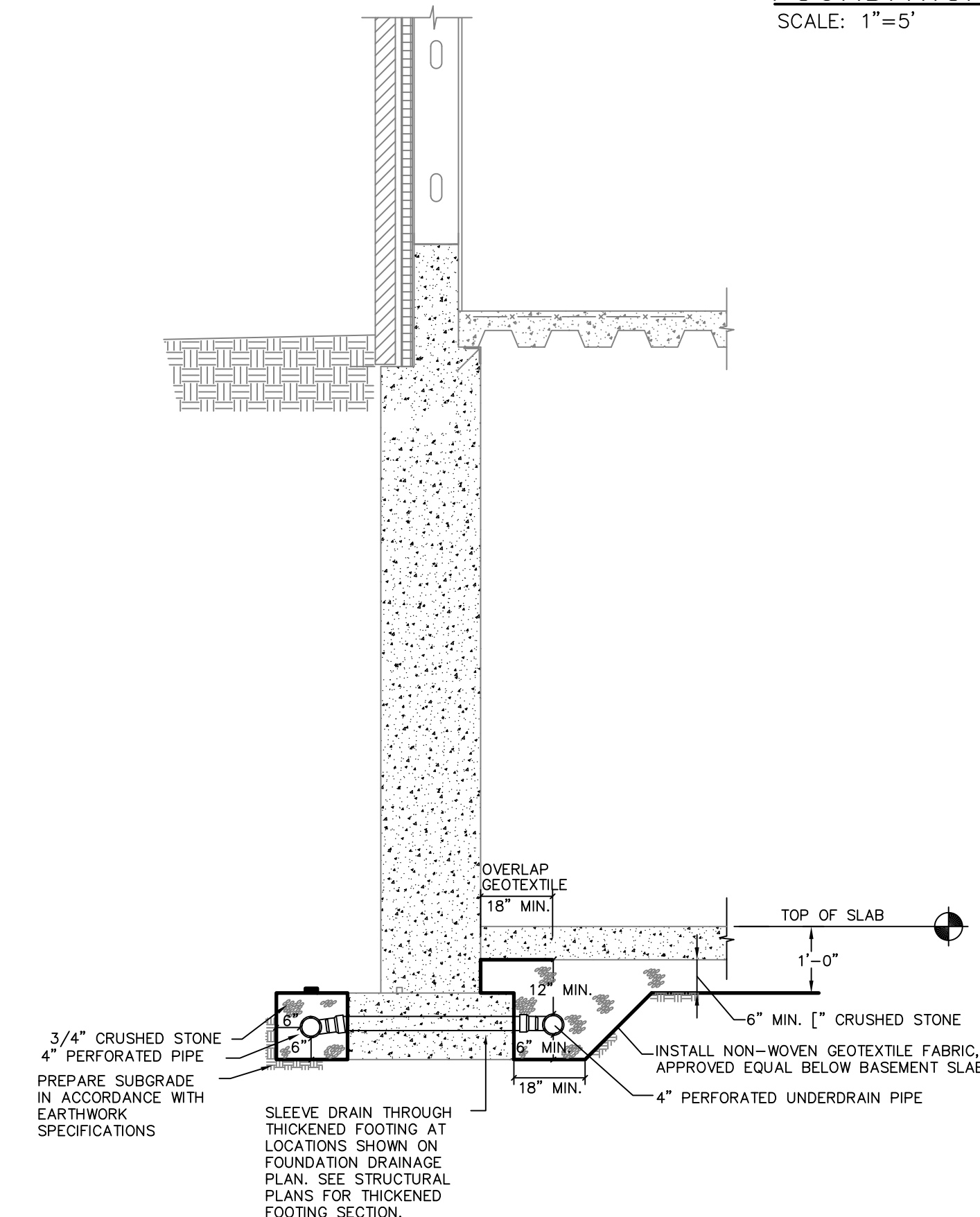
TYPICAL PERIMETER DRAIN INSTALLATION SCALE: 1/2"=1'
