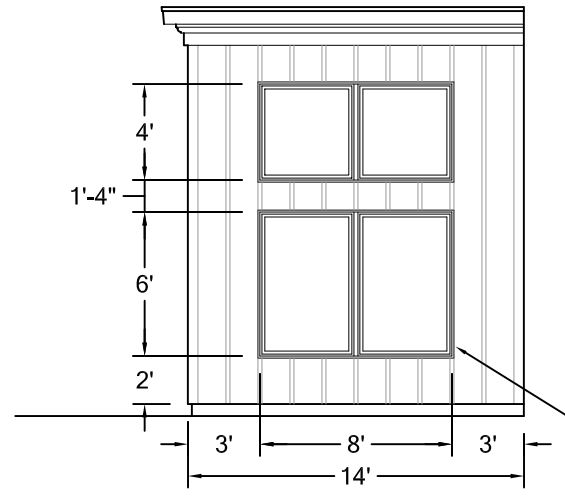
2 RETURN ELEVATION @ LEFT SCALE: 1/8"=1'-0"
