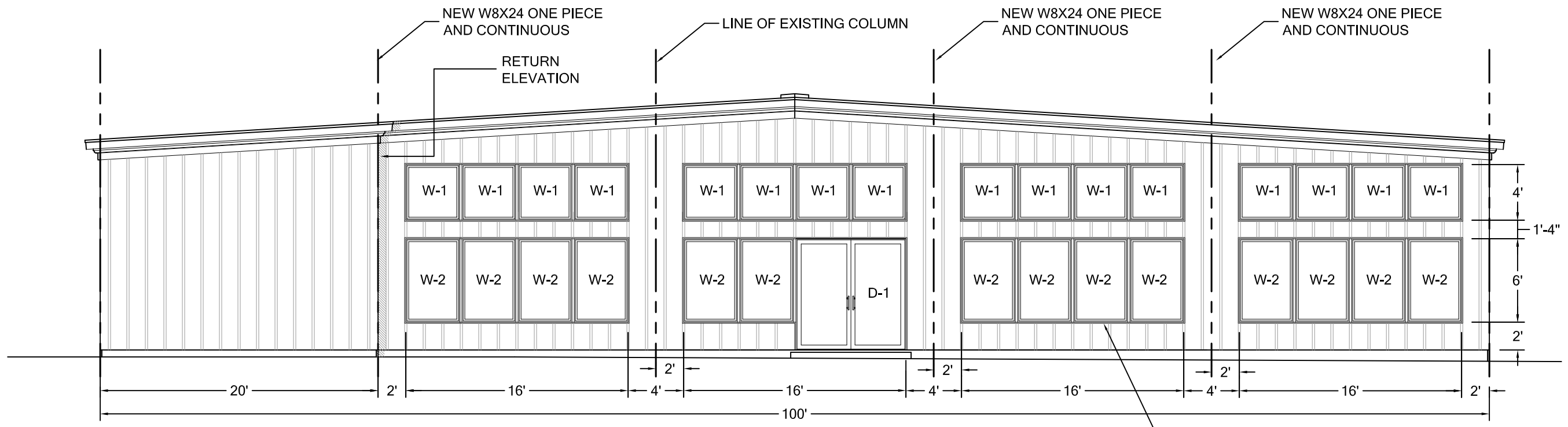
1 FRONT ELEVATION - STORE FRONT SCALE: 1/8"=1'-0"
