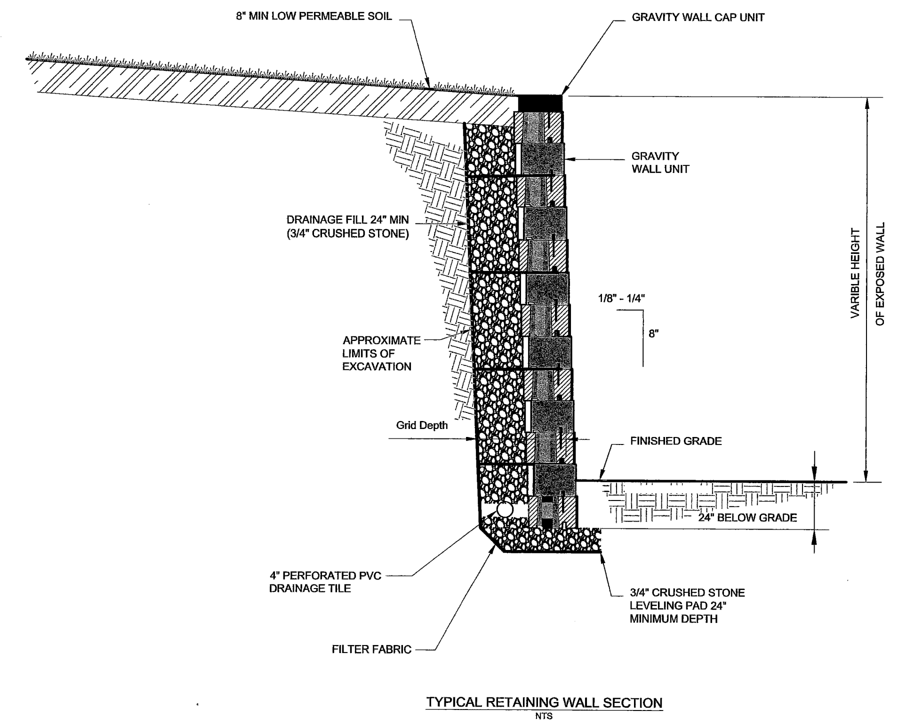
TYPICAL RETAINING WALL SECTION NOT TO SCALE
