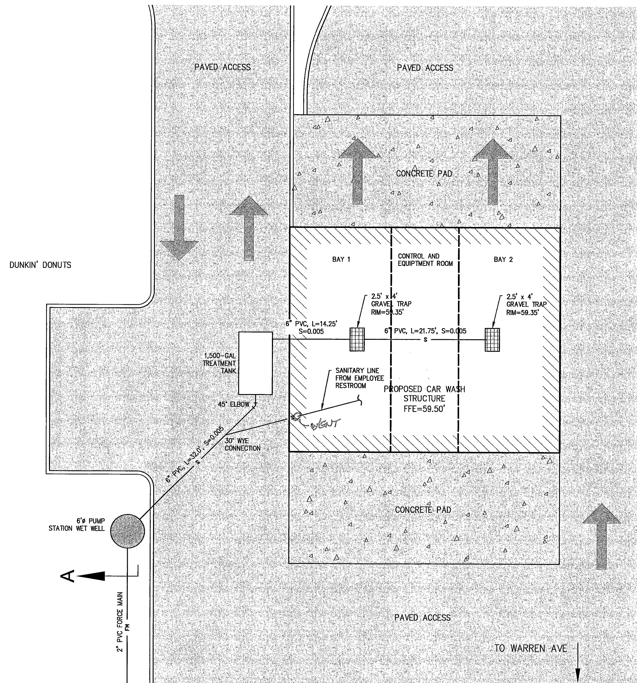
SANITARY SEWER LAYOUT: SECTION A-A 1"=10'
