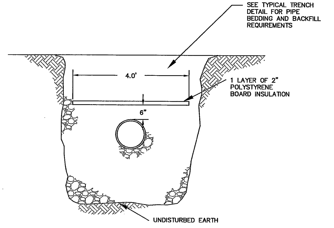
INSULATED PIPE TRENCH DETAIL NOT TO SCALE
