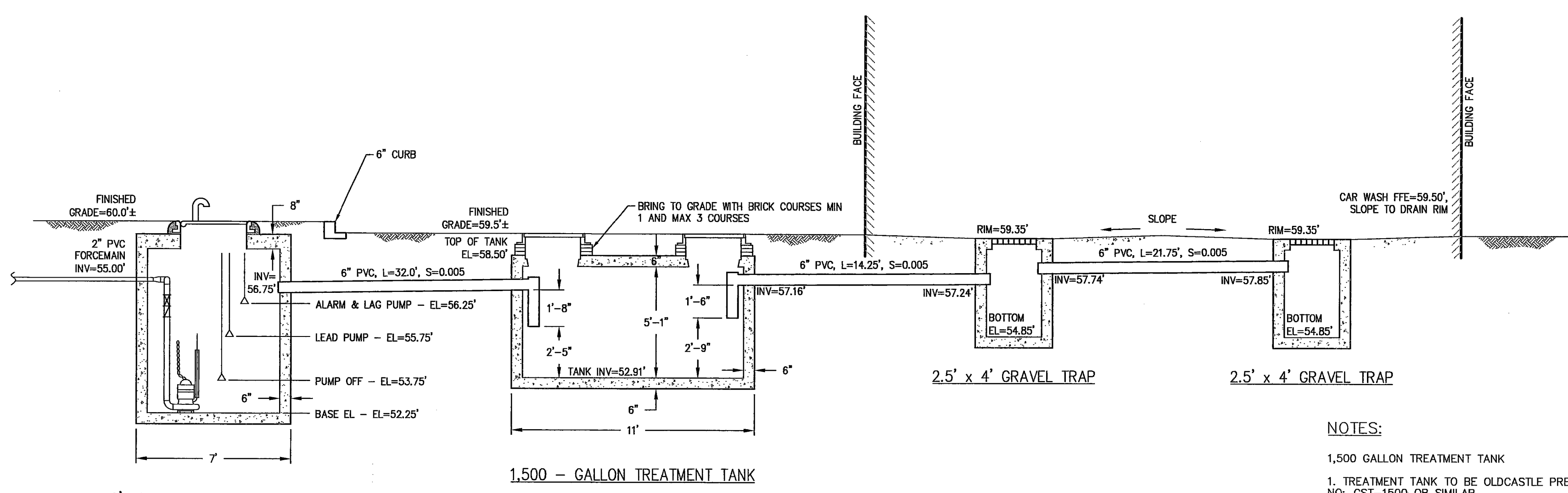
SECTION PUMP STATION WET WELL & DETAIL NOT TO SCALE
