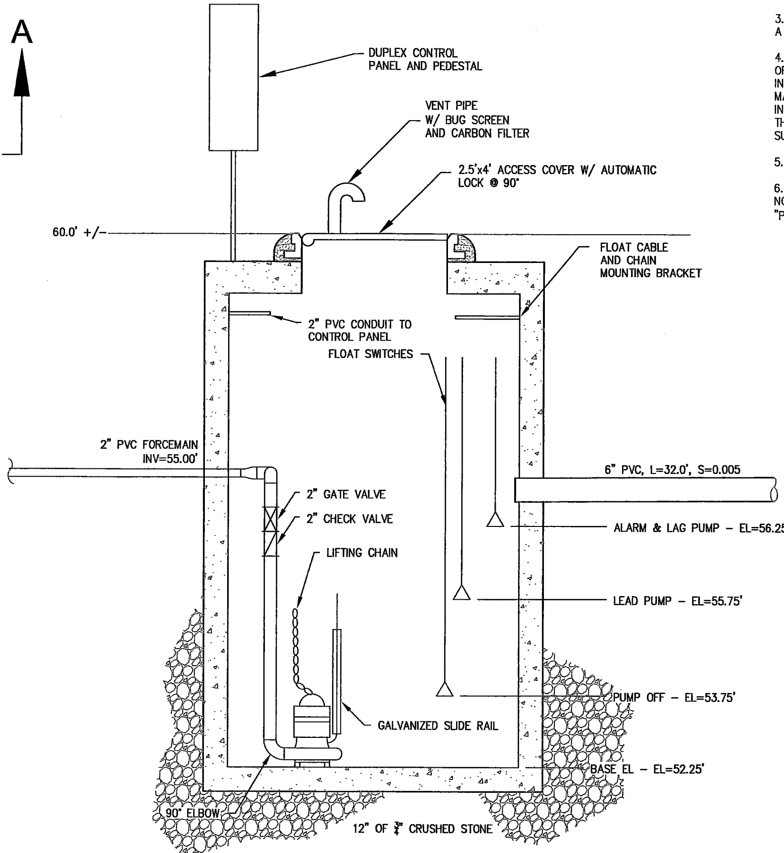
SECTION PUMP STATION WET WELL & DETAIL NOT TO SCALE
