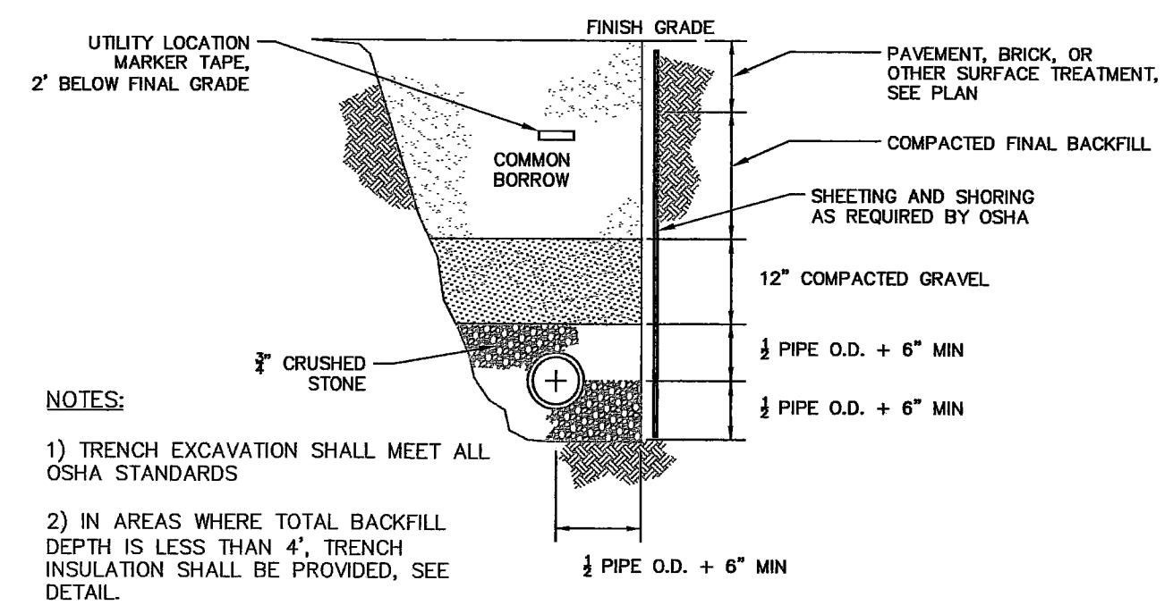
TYPICAL PIPE TRENCH DETAIL NOT TO SCALE
